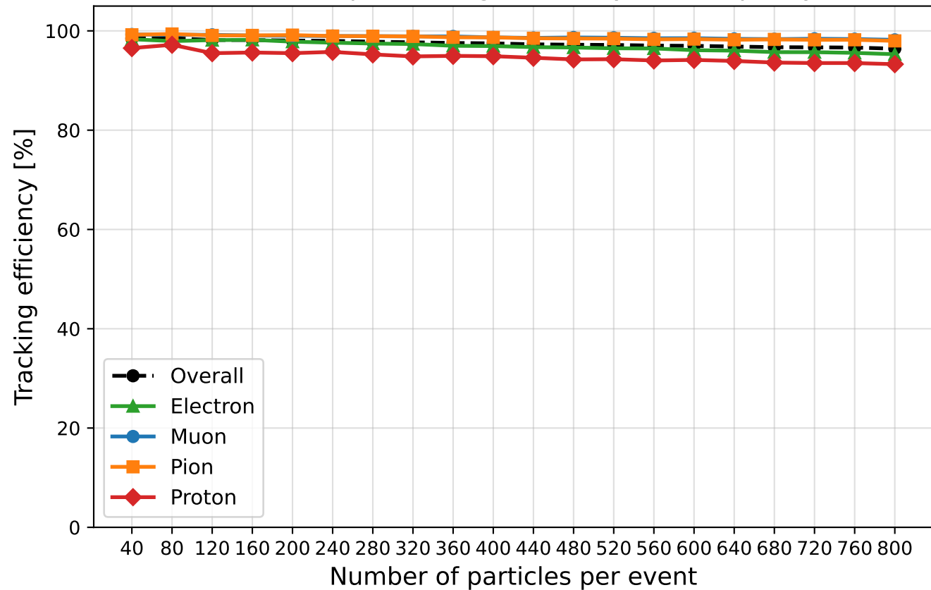
OOD Sweep: Tracking Efficiency vs Multiplicity
