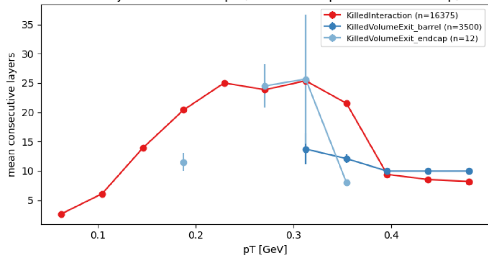
Mean layers traversed vs pT (volume-exit split: barrel vs endcap)
