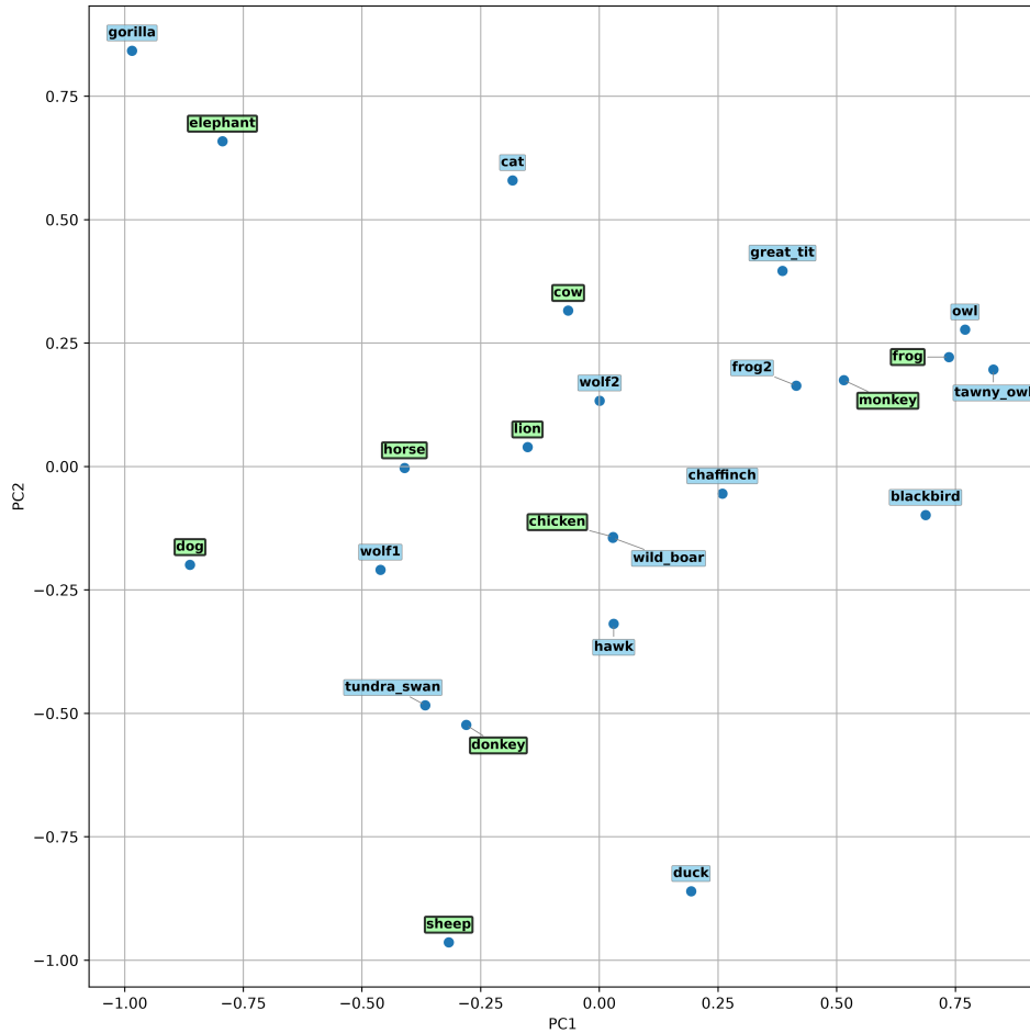
Figure 6: Samples in the space of the first two principal components (PC1 and PC2); green labels with a black border denote sounds from the MLT set [11].
