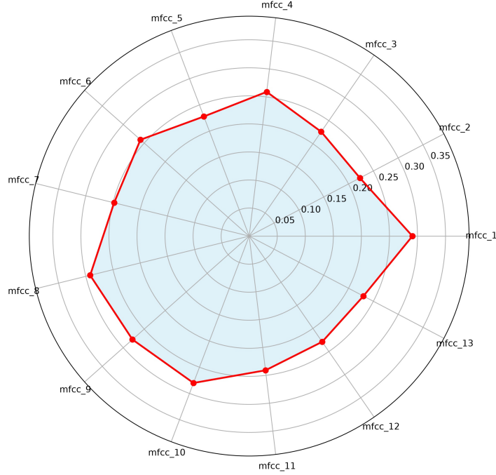
Figure 4: Standard deviation of the MFCCs.
