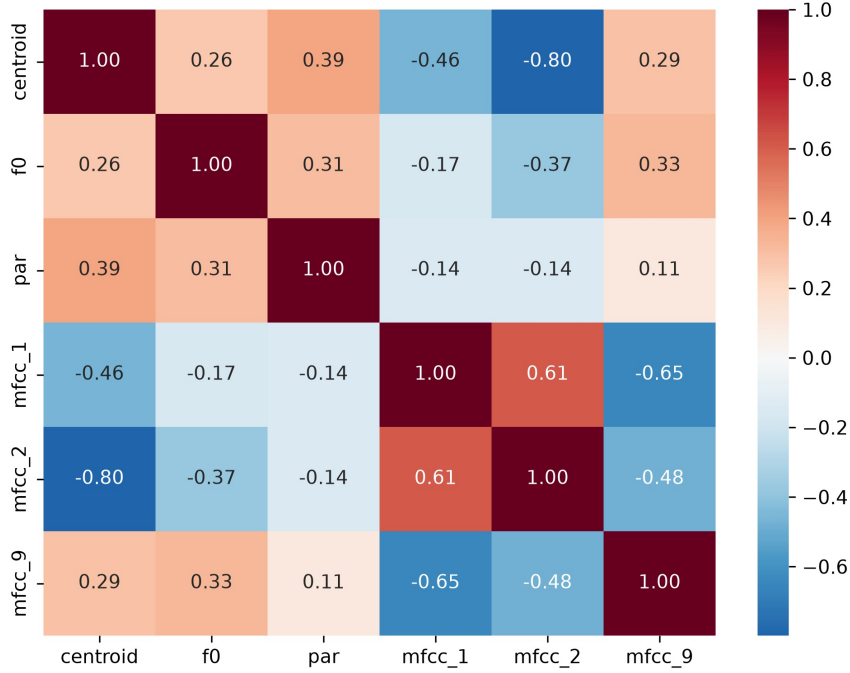
Figure 5: Correlation matrix for six selected acoustic descriptors: spectral centroid, F0, PAR, MFCC_1, MFCC_2, and MFCC_9. Each cell represents the correlation between a pair of descriptors across the analyzed sound samples. The displayed subset is used to examine relationships among features; the PCA was performed separately using the full 16-dimensional feature vector.
