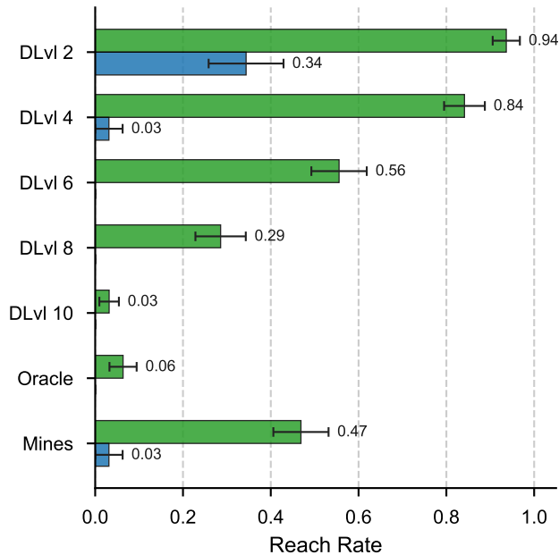
NetHack: Milestone Reach
