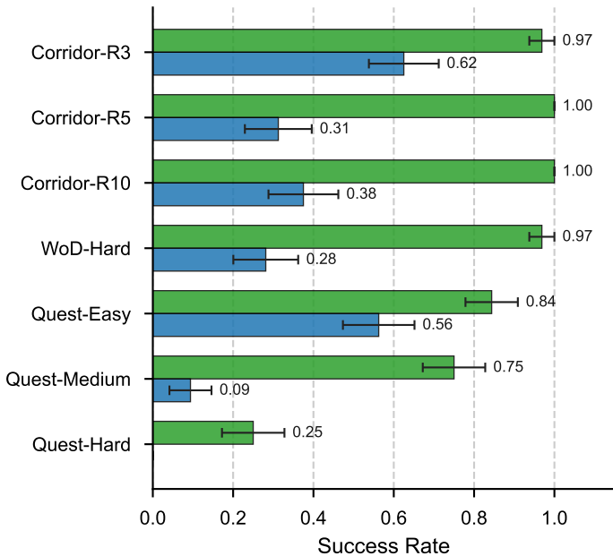
MiniHack: Success Rate
