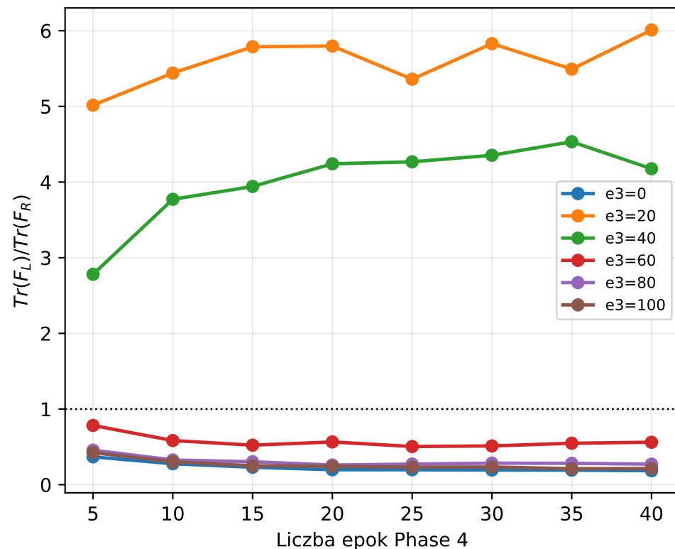
seed 184
