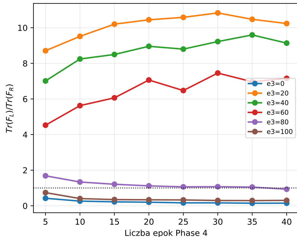
seed 83
