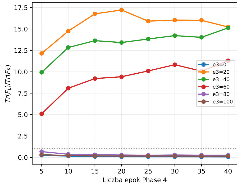
seed 285
