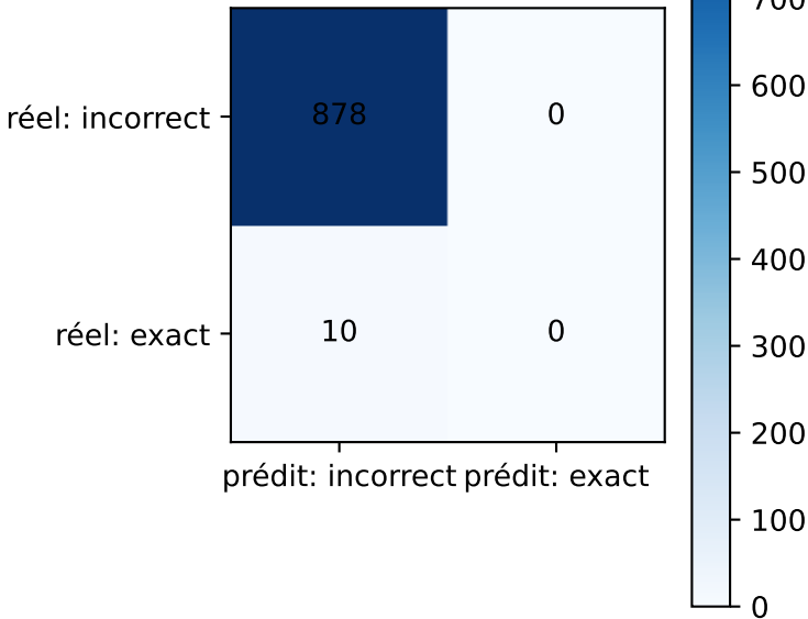
Matrice de confusion (Random Forest)
