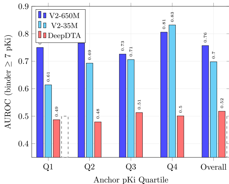
(C) AUROC (binder threshold pKi \geq 7 ) by Quartile
