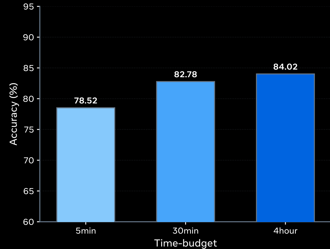
Agentic RPM
