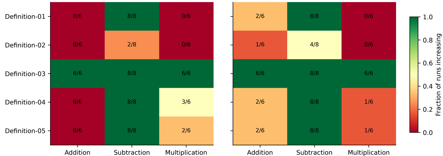
Train examples
