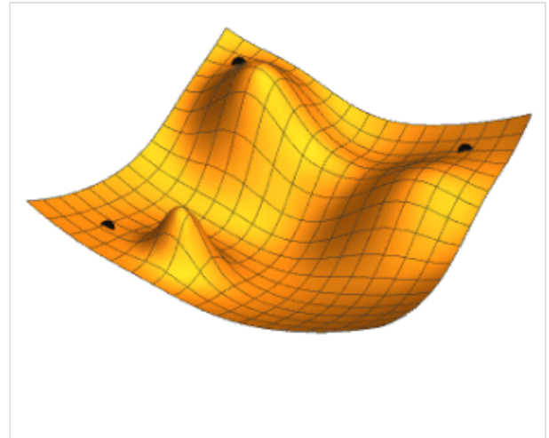
Illustration of gradient descent for three different starting points; two parameters (represented by the plan coordinates) are adjusted in order to minimise the loss function (the height).
