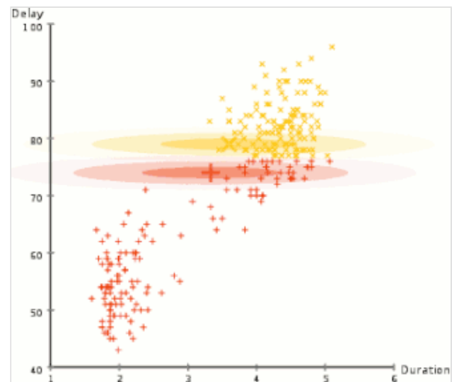
Expectation–maximisation clustering of Old Faithful eruption data starts from a random guess but then successfully converges on an accurate clustering of the two physically distinct modes of eruption.
