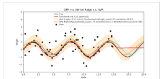
An example of Gaussian Process Regression (prediction) compared with other regression models [105]
