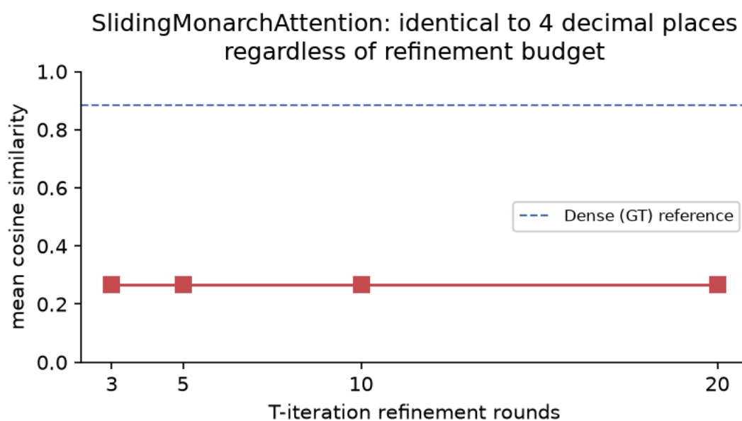
Figure 5. SlidingMonarchAttention: retrieval quality is identical to four decimal places across T=3, 5, 10 , and 20 refinement iterations—a structural ceiling, not a refinement-budget problem.
