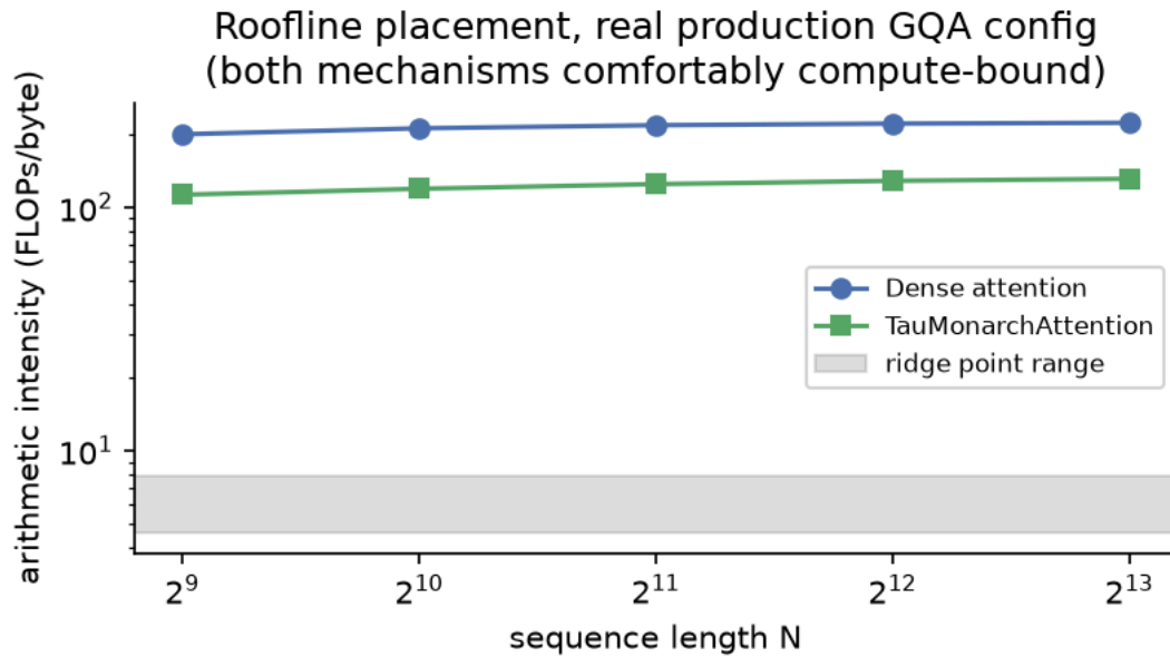
Figure 10. Implied arithmetic intensity of dense attention and TauMonarchAttention at the real production GQA configuration, against the 5500U's estimated compute/memory ridge point. Both mechanisms sit well above the ridge across the project's target sequence lengths.
