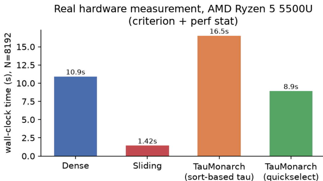
Figure 9. Real hardware wall-clock, N=8192 , AMD Ryzen 5 5500U. The sort-based \tau implementation is slower than dense attention; replacing it with quickselect (mathematically identical \tau value) recovers a genuine 1.22\times win.
