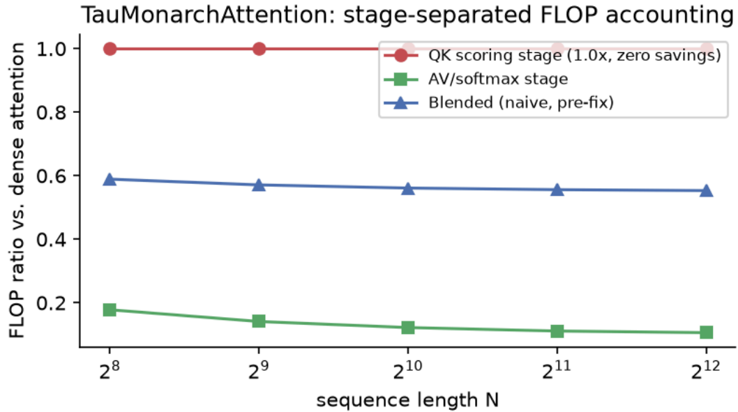
Figure 7. Stage-separated FLOP accounting: QK scoring gets zero savings versus dense (a structural property, not an implementation gap); the AV/softmax stage benefits from the survivor rate; the naive pre-fix blended estimate is shown for reference against Section 7.2's correction.
