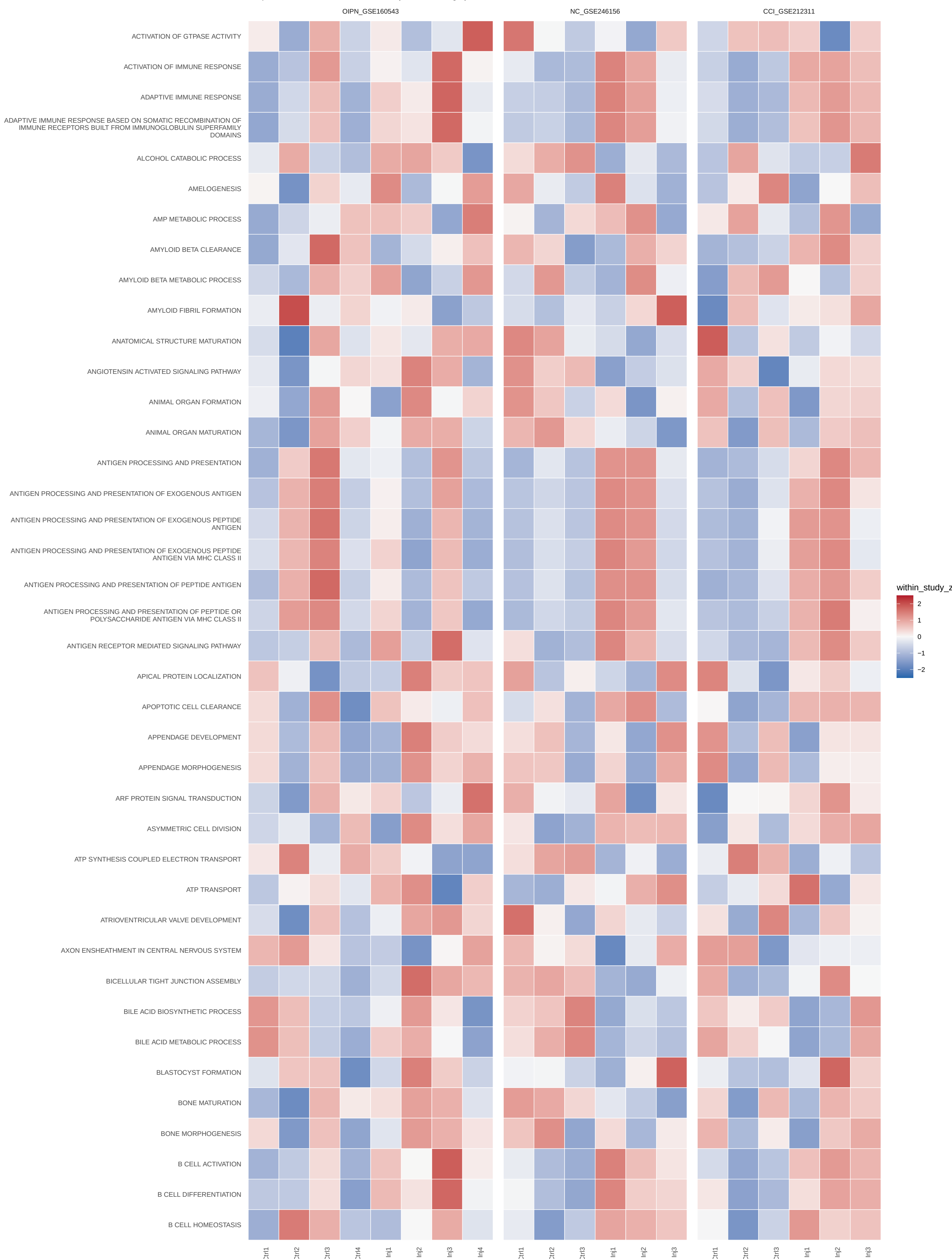
GO:BP sample-level GSVA; within-study z scores Independent DRG cohorts; * within-study FDR <0.05; gray = unavailable
