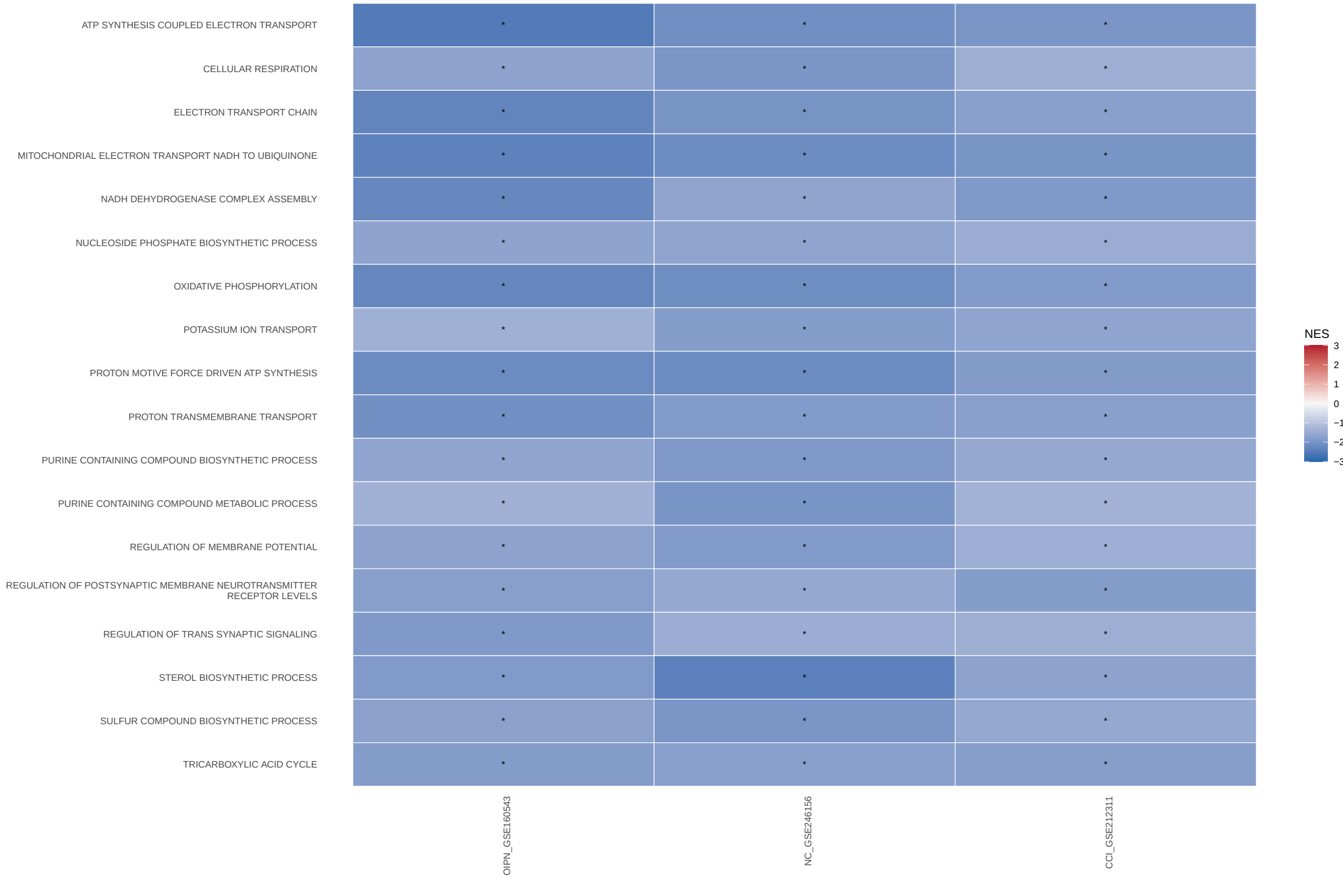
GO:BP shared_negative Independent DRG cohorts; * within-study FDR <0.05; gray = unavailable
