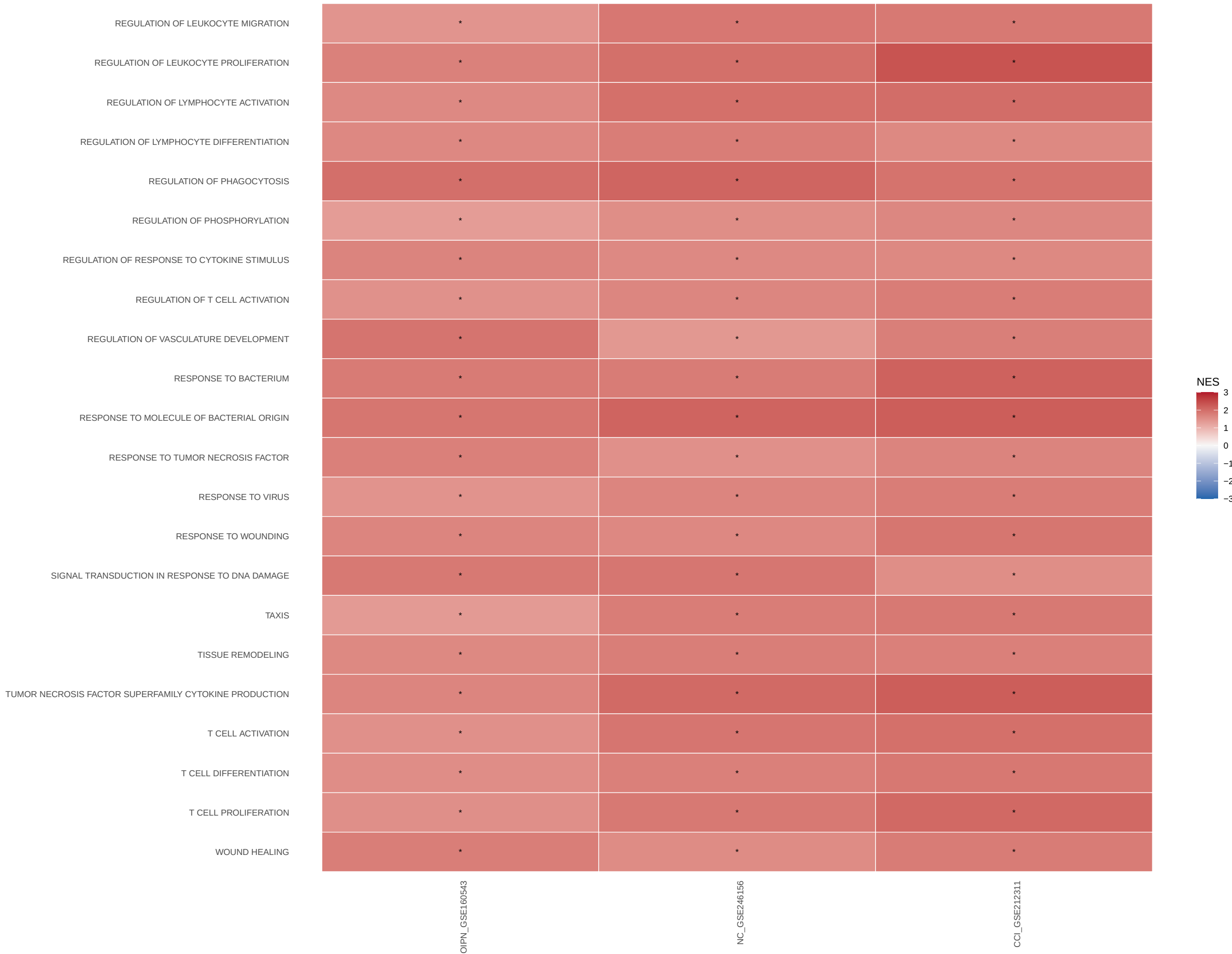
GO:BP shared_positive Independent DRG cohorts; * within-study FDR <0.05; gray = unavailable
