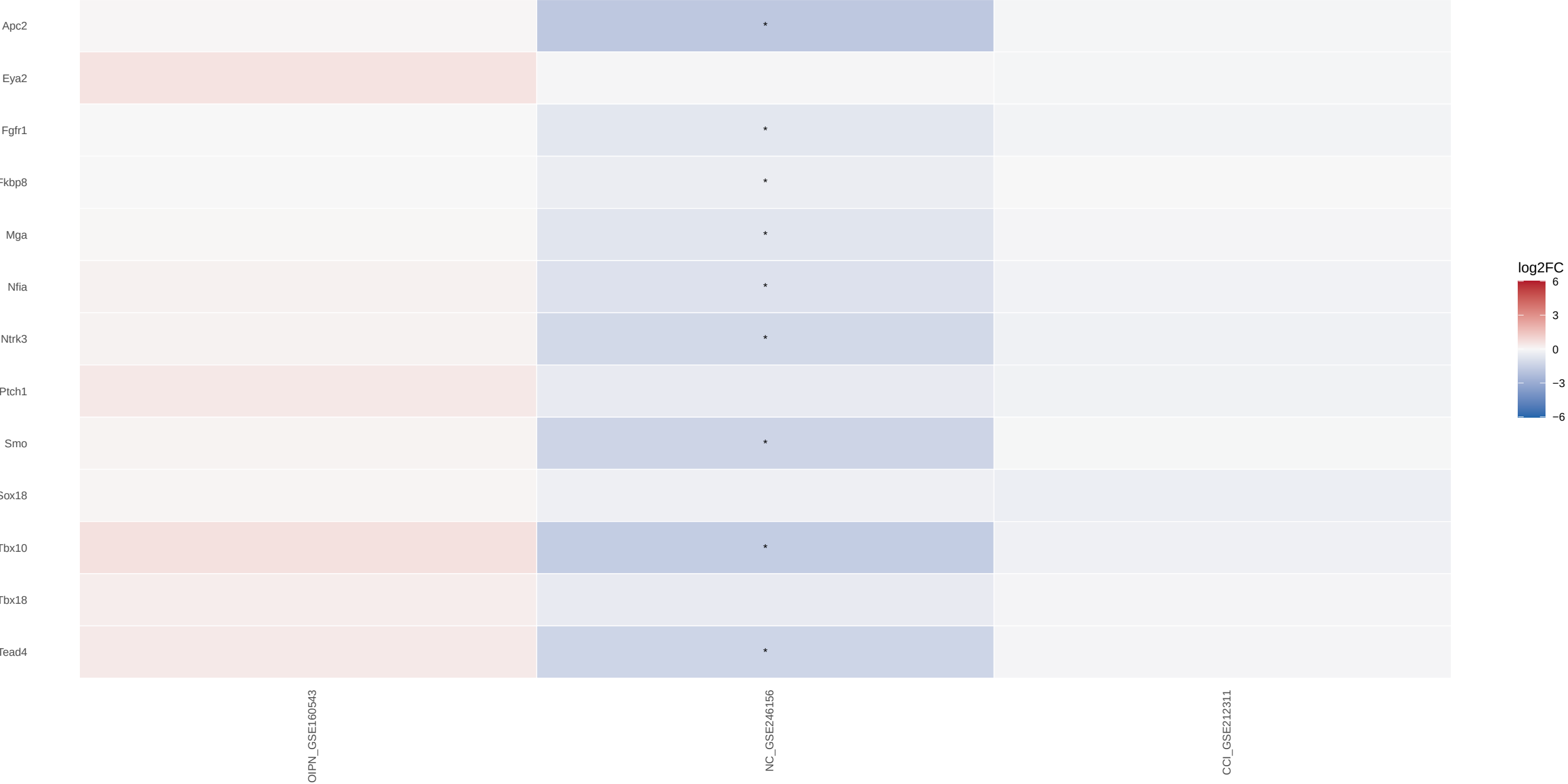
CELL FATE SPECIFICATION gene log2FC Independent DRG cohorts; * within-study FDR <0.05; gray = unavailable
