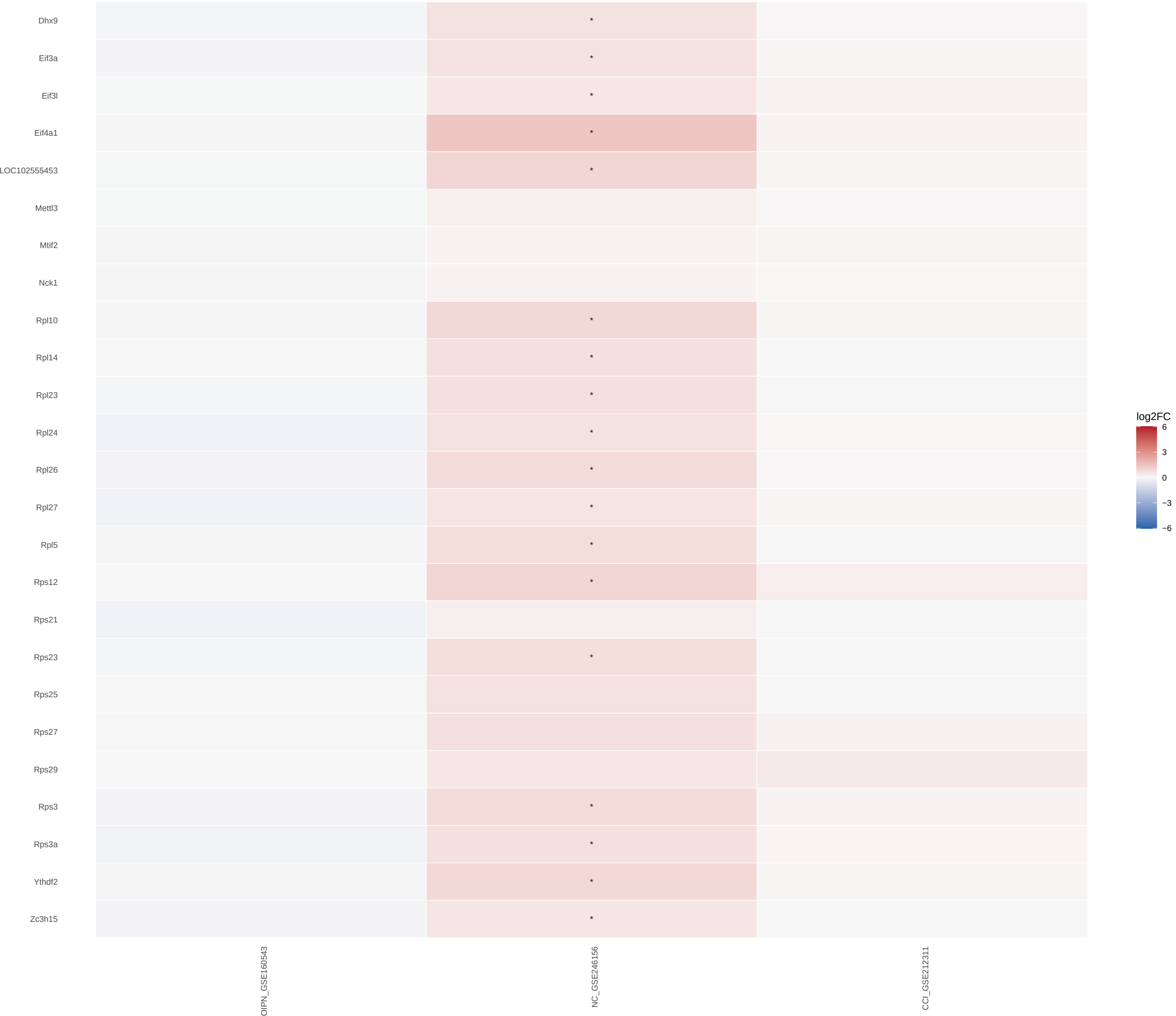
CYTOPLASMIC TRANSLATION gene log2FC Independent DRG cohorts; * within-study FDR <0.05; gray = unavailable
