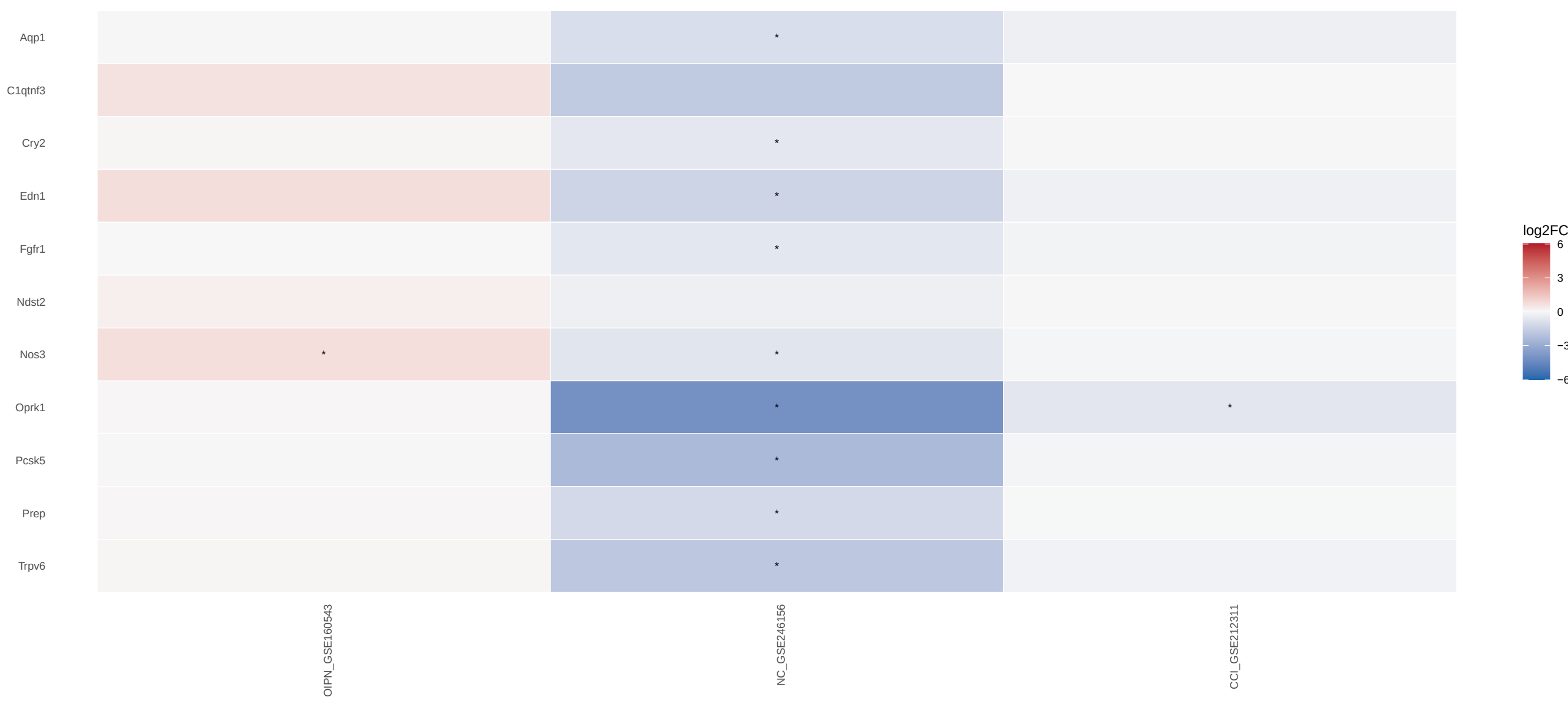
ENDOCRINE PROCESS gene log2FC Independent DRG cohorts; * within-study FDR <0.05; gray = unavailable
