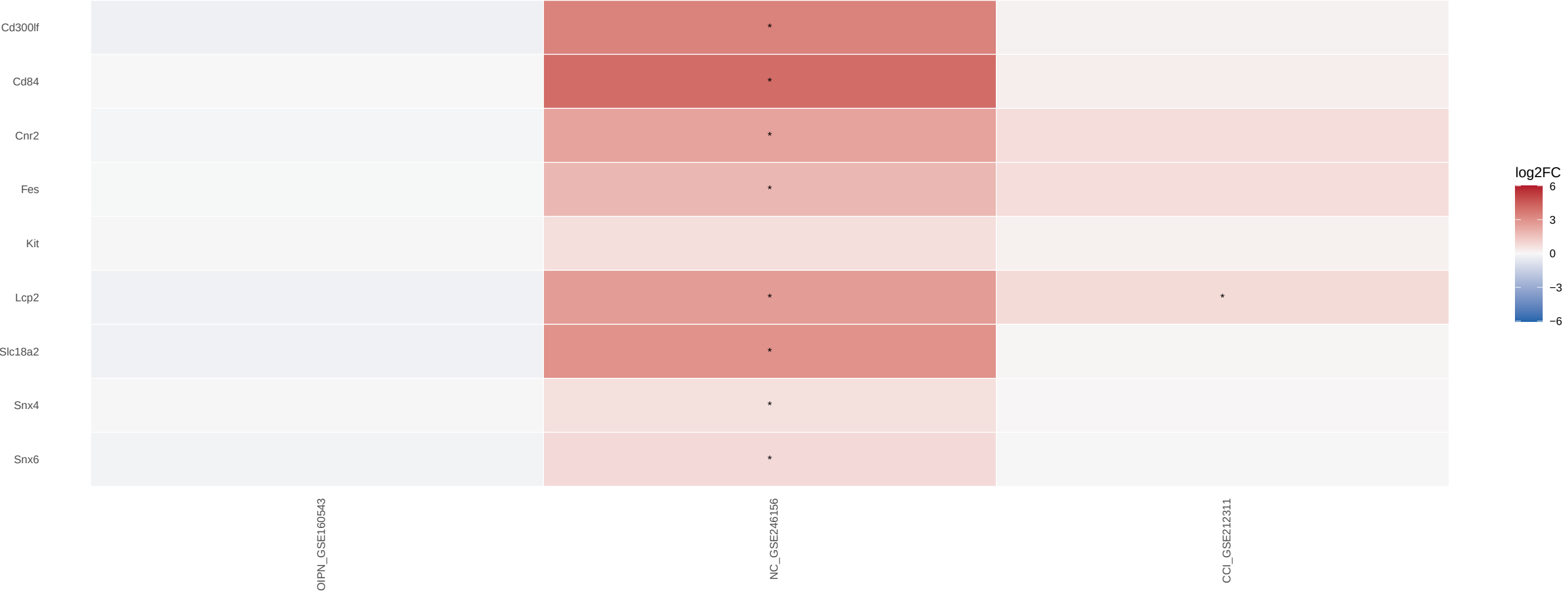
MAST CELL ACTIVATION gene log2FC Independent DRG cohorts; * within-study FDR <0.05; gray = unavailable
