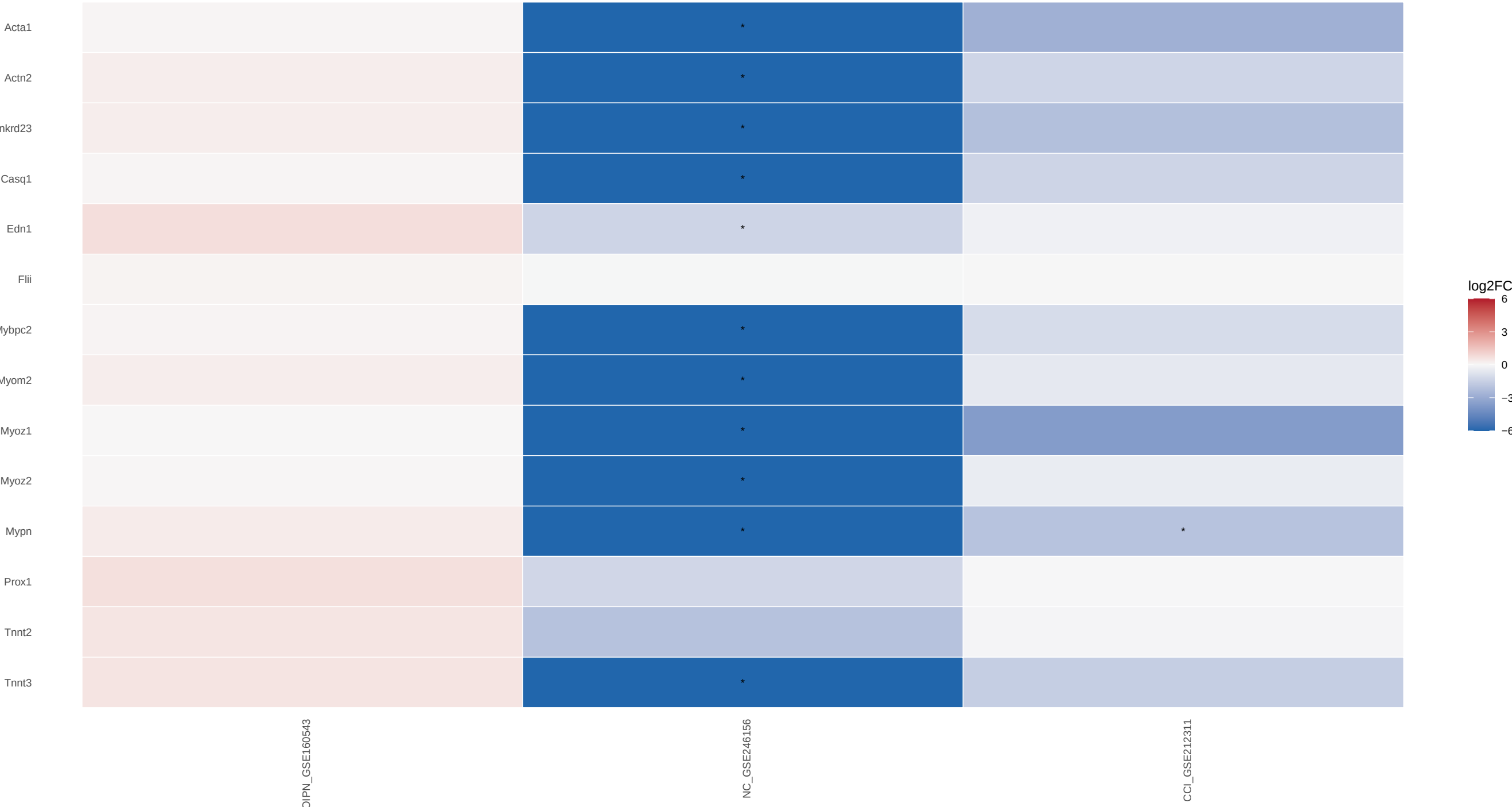
MYOFIBRIL ASSEMBLY gene log2FC Independent DRG cohorts; * within-study FDR <0.05; gray = unavailable
