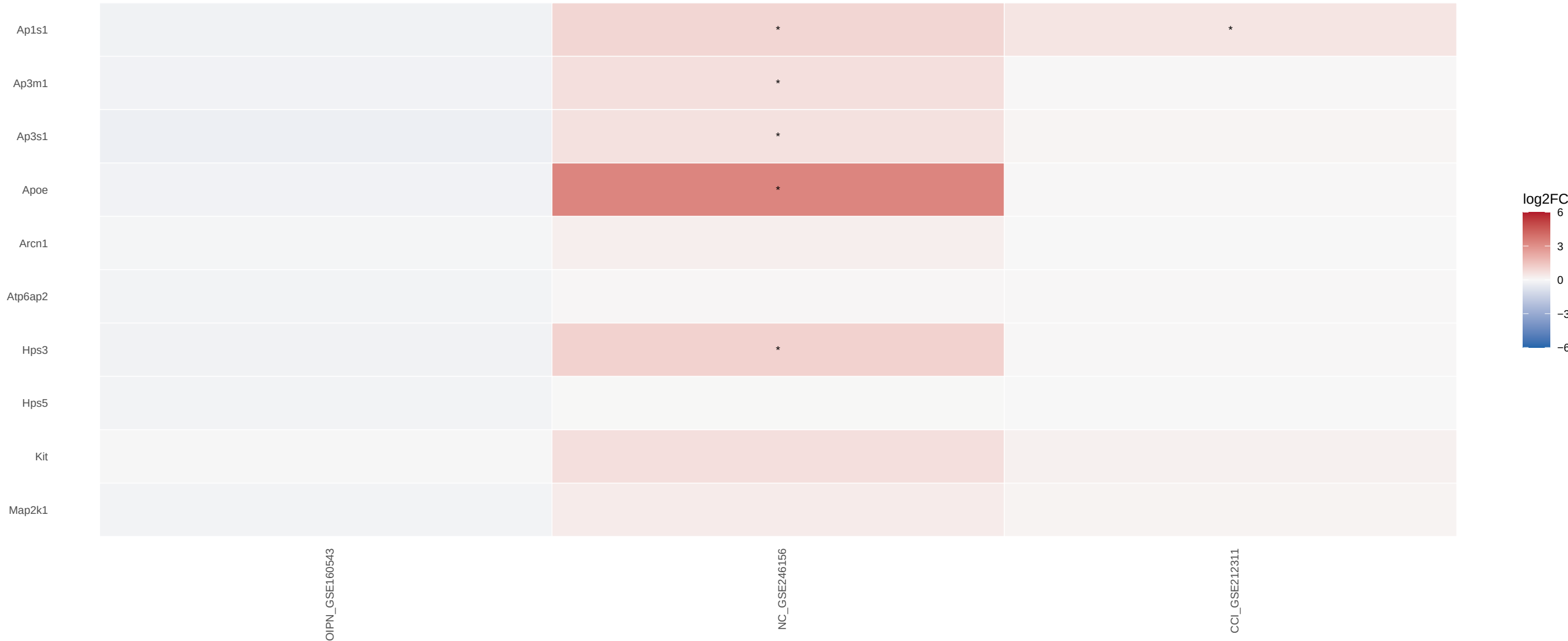
PIGMENTATION gene log2FC Independent DRG cohorts; * within-study FDR <0.05; gray = unavailable
