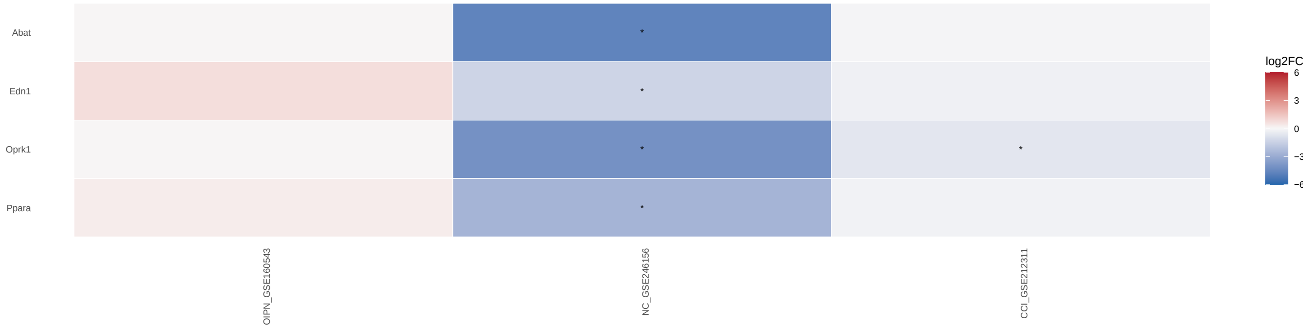
RESPONSE TO NICOTINE gene log2FC Independent DRG cohorts; * within-study FDR <0.05; gray = unavailable
