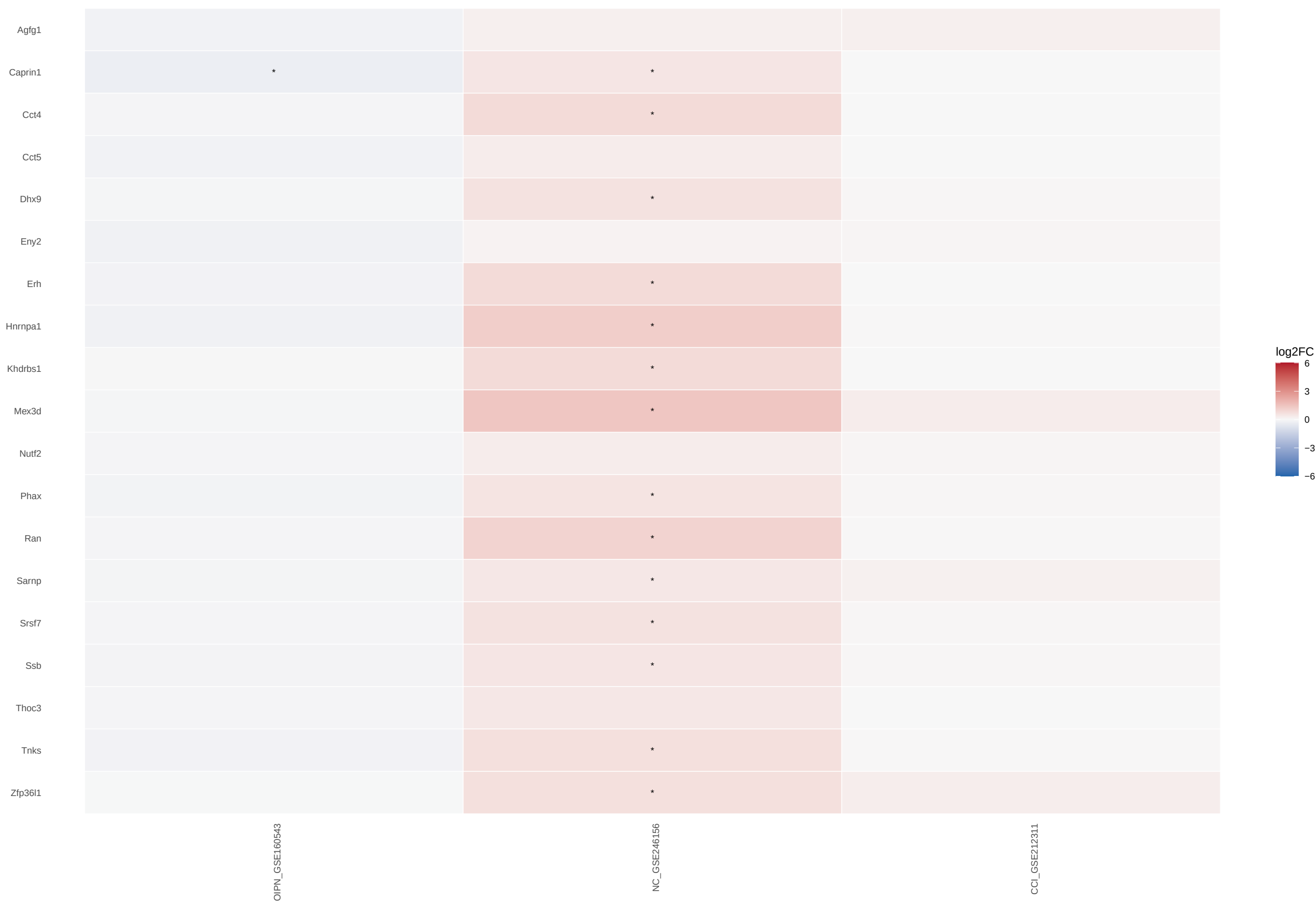
RNA LOCALIZATION gene log2FC Independent DRG cohorts; * within-study FDR <0.05; gray = unavailable
