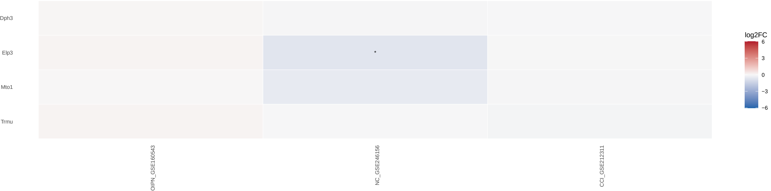
TRNA WOBBLE BASE MODIFICATION gene log2FC Independent DRG cohorts; * within-study FDR <0.05; gray = unavailable
