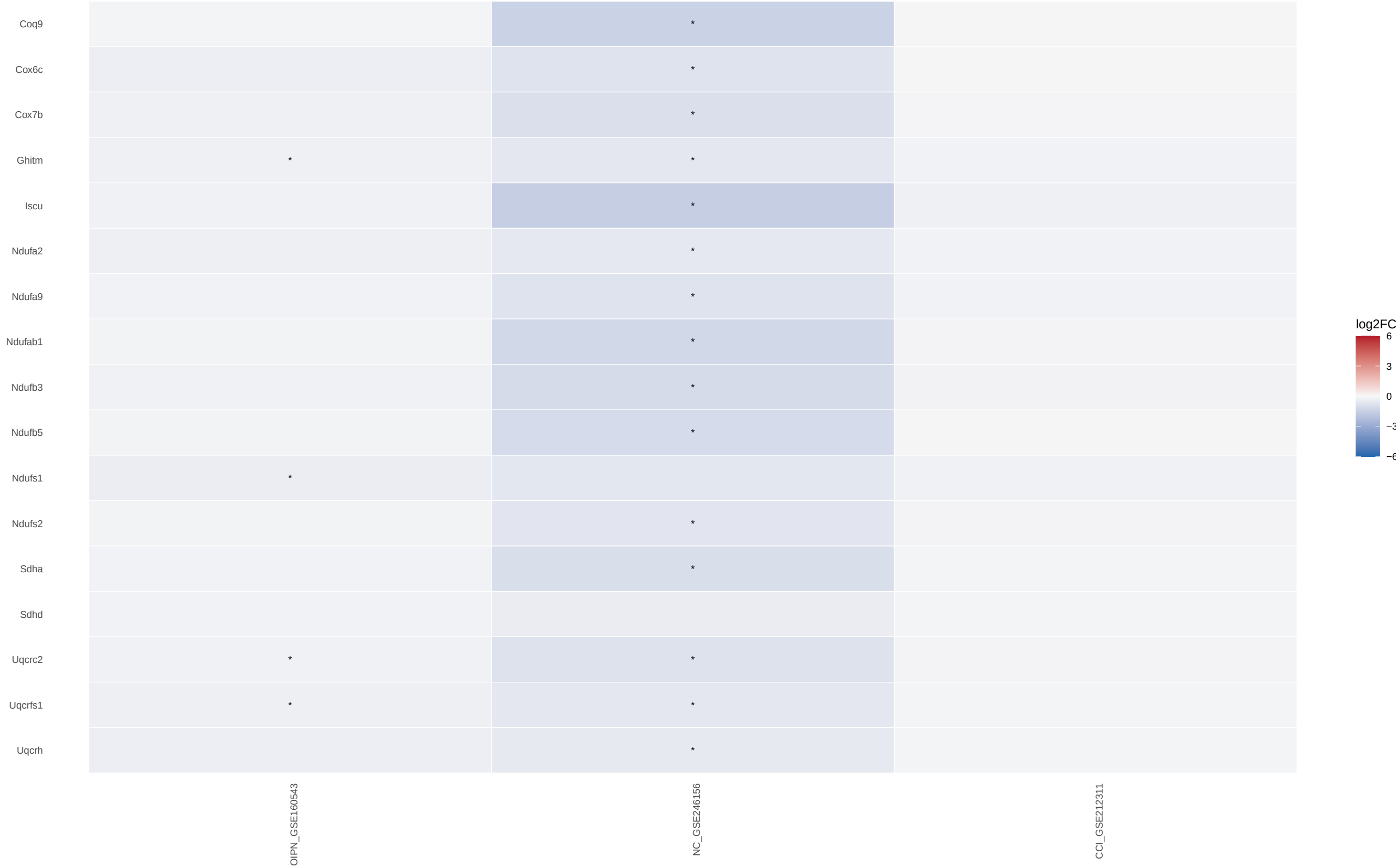
ATP SYNTHESIS COUPLED ELECTRON TRANSPORT gene log2FC Independent DRG cohorts; * within-study FDR <0.05; gray = unavailable
