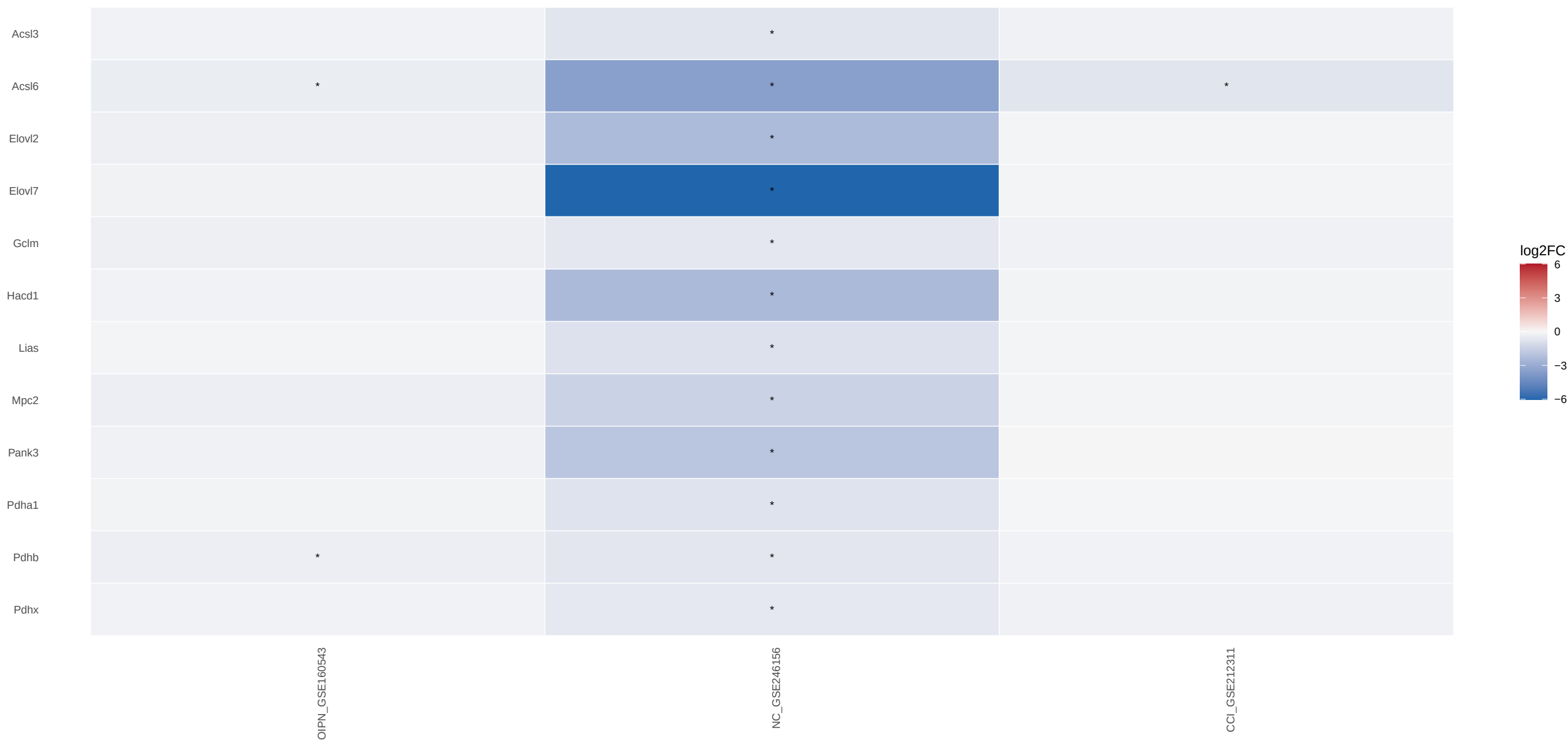
SULFUR COMPOUND BIOSYNTHETIC PROCESS gene log2FC Independent DRG cohorts; * within-study FDR <0.05; gray = unavailable
