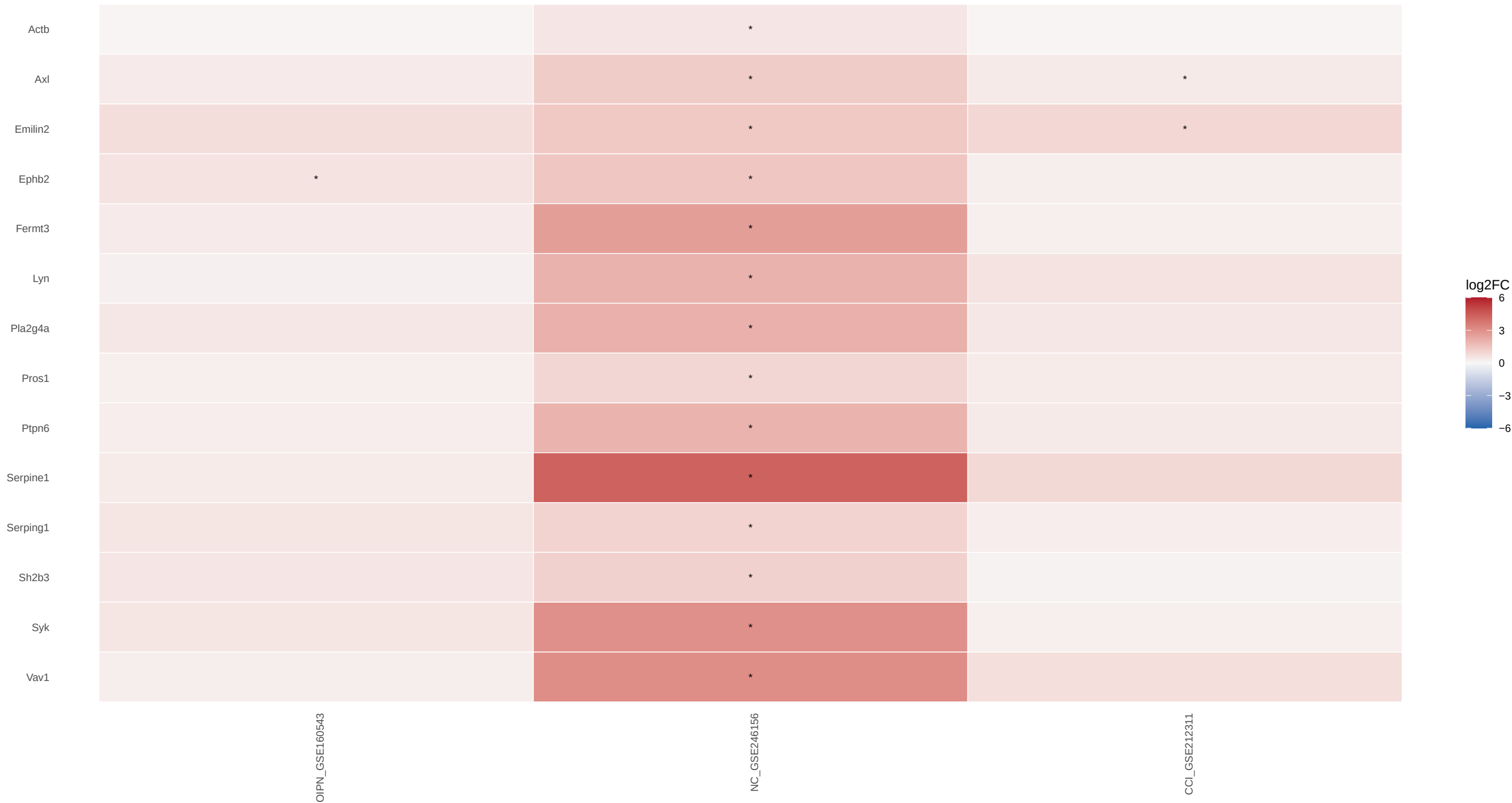
HEMOSTASIS gene log2FC Independent DRG cohorts; * within-study FDR <0.05; gray = unavailable
