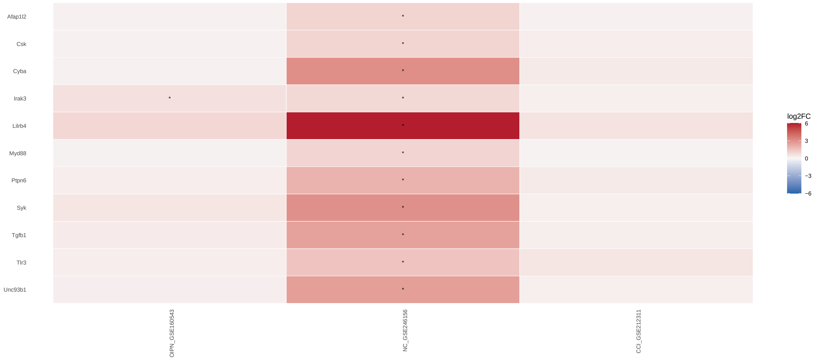
INTERLEUKIN 6 PRODUCTION gene log2FC Independent DRG cohorts; * within-study FDR <0.05; gray = unavailable
