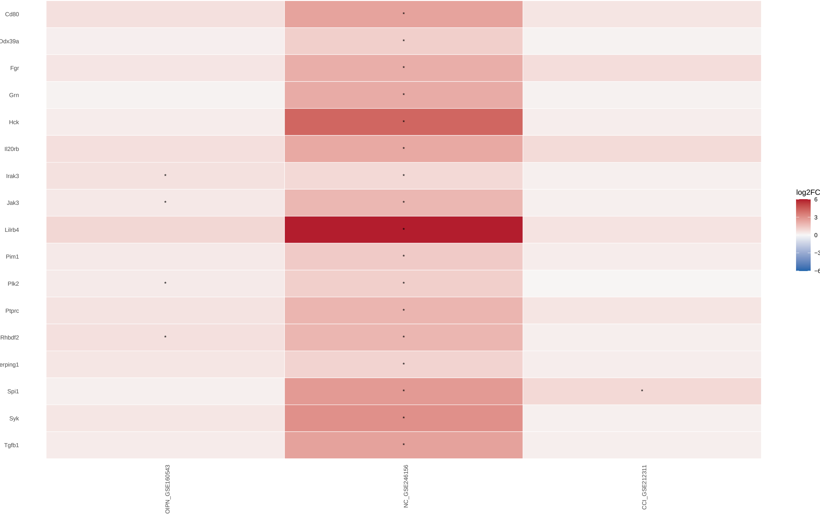
NEGATIVE REGULATION OF IMMUNE RESPONSE gene log2FC Independent DRG cohorts; * within-study FDR <0.05; gray = unavailable
