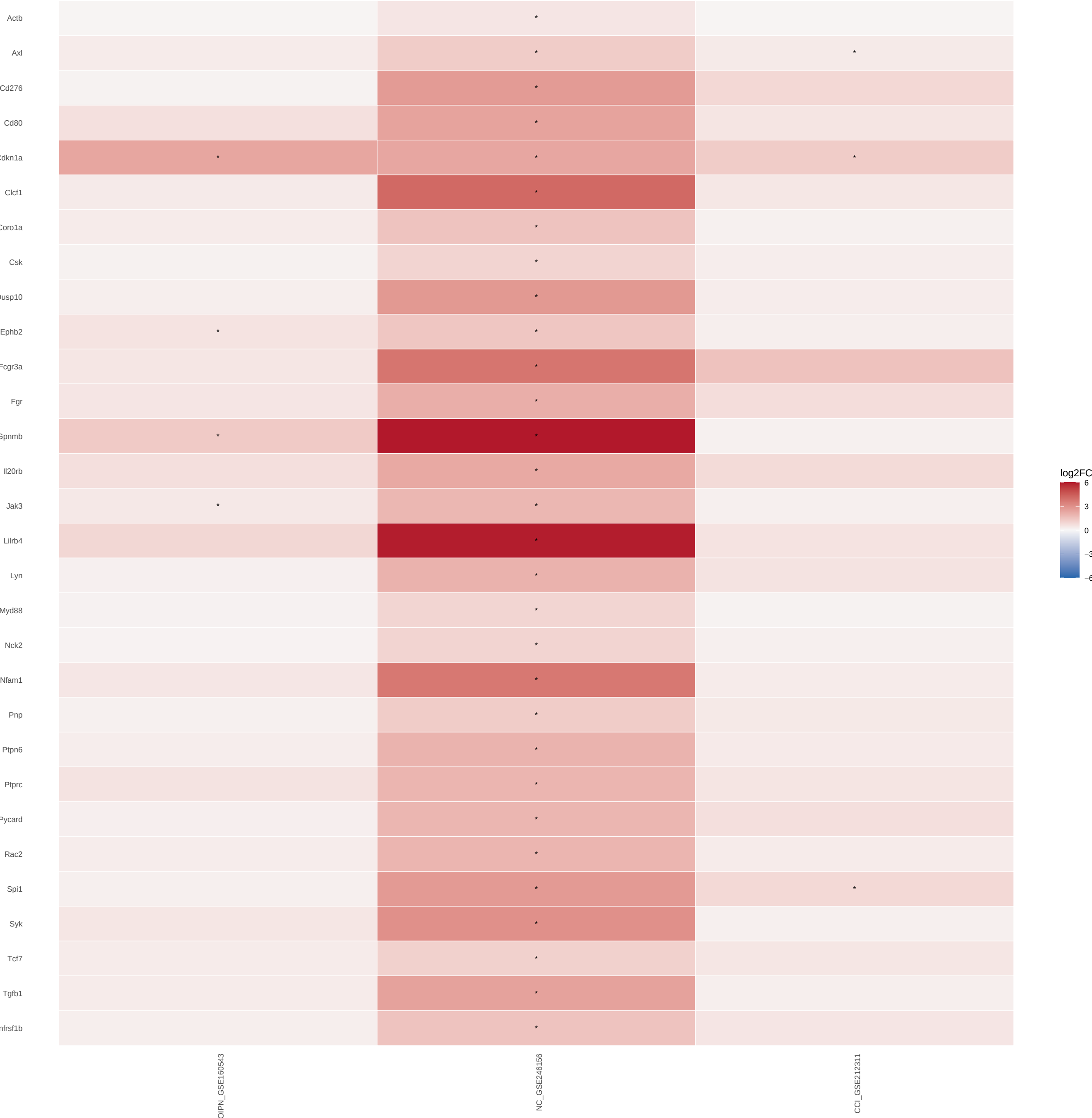
REGULATION OF LYMPHOCYTE ACTIVATION gene log2FC Independent DRG cohorts; * within-study FDR <0.05; gray = unavailable
