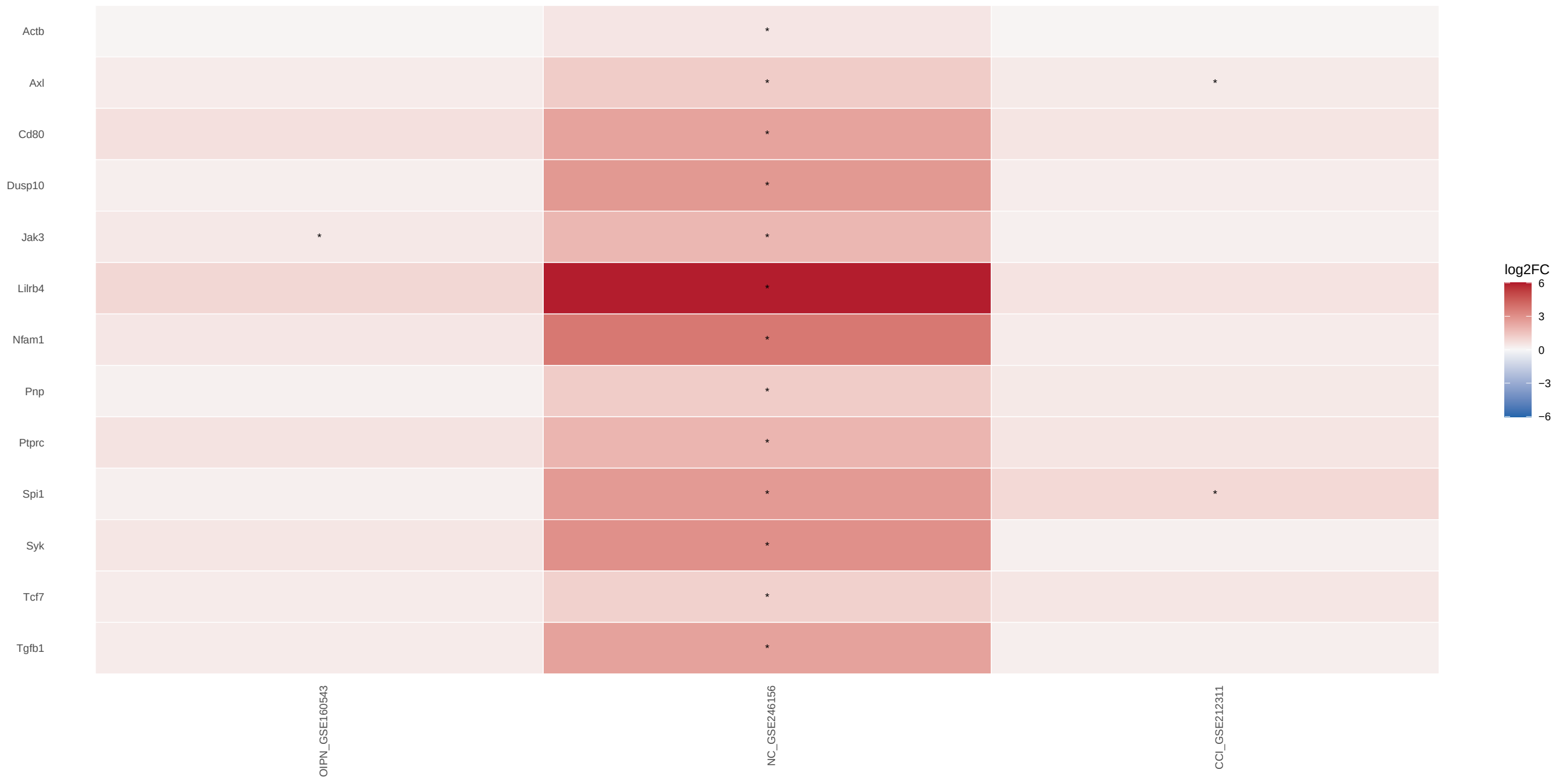
REGULATION OF LYMPHOCYTE DIFFERENTIATION gene log2FC Independent DRG cohorts; * within-study FDR <0.05; gray = unavailable
