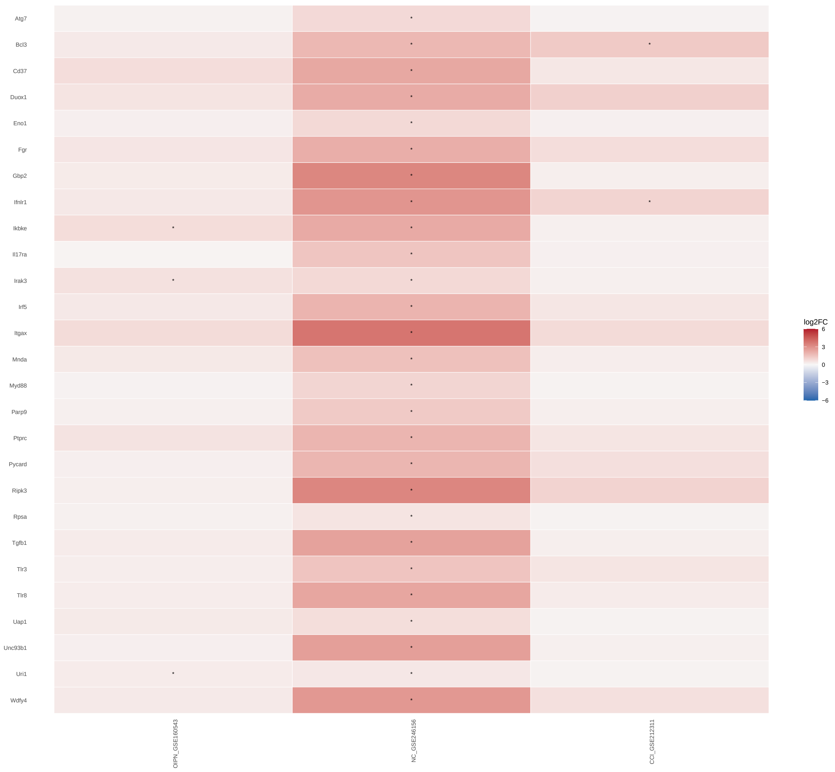
RESPONSE TO VIRUS gene log2FC Independent DRG cohorts; * within-study FDR <0.05; gray = unavailable
