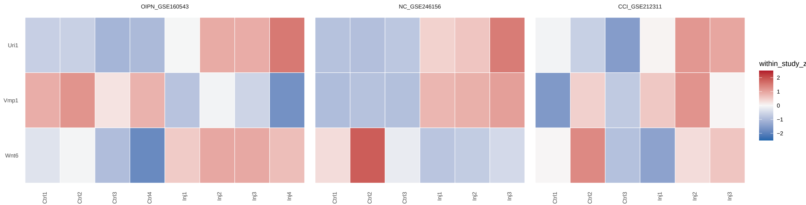
GO:BP priority genes: sample-level expression Independent DRG cohorts; * within-study FDR <0.05; gray = unavailable
