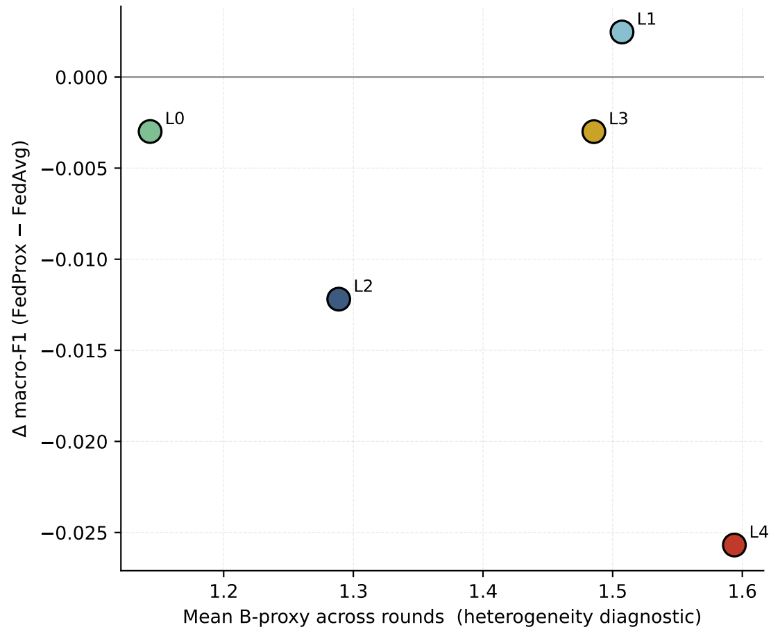
(b) Higher B \rightarrow FedProx advantage? (Spearman r = -0.30 , p = 0.62 )
