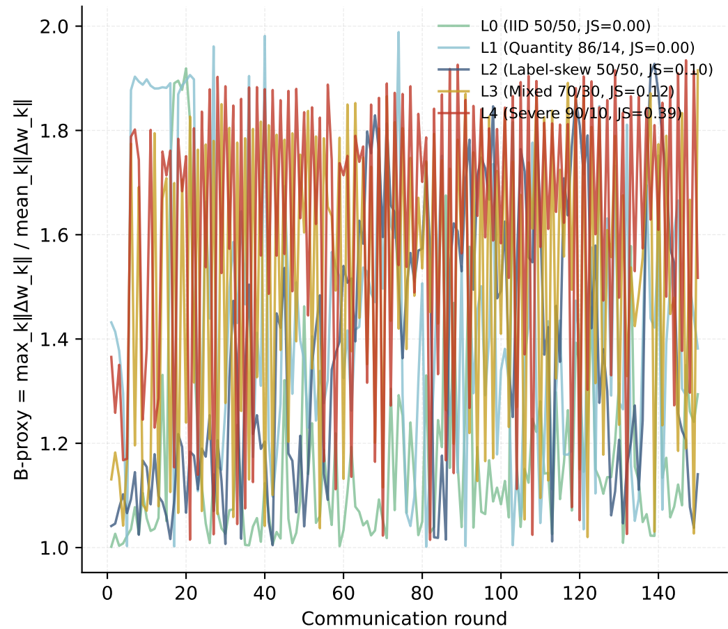
(a) B-dissimilarity proxy trajectories — FedAvg, seed 42
