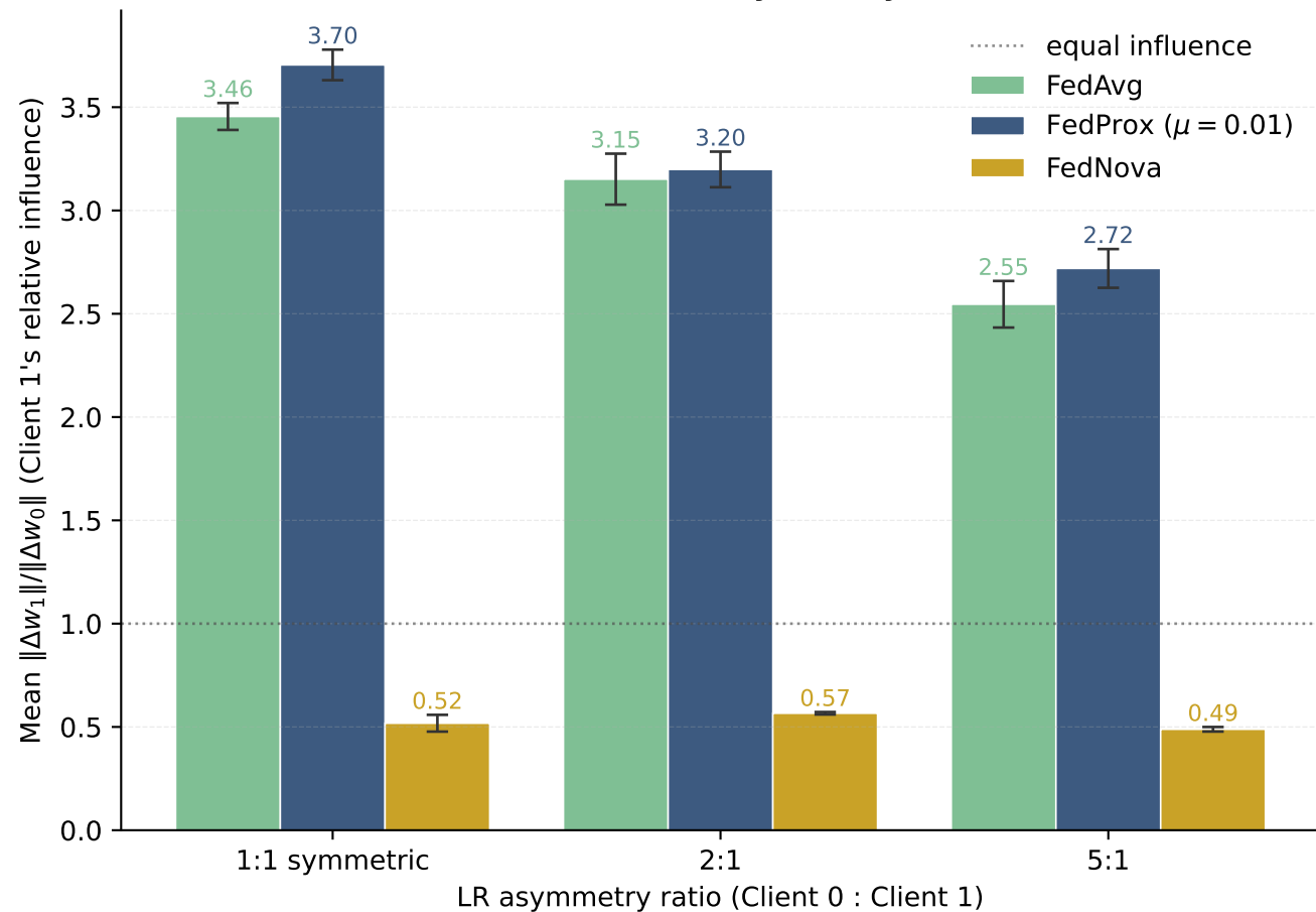
Per-client influence ratio across LR asymmetry — how much does each client contribute to the aggregate update?
