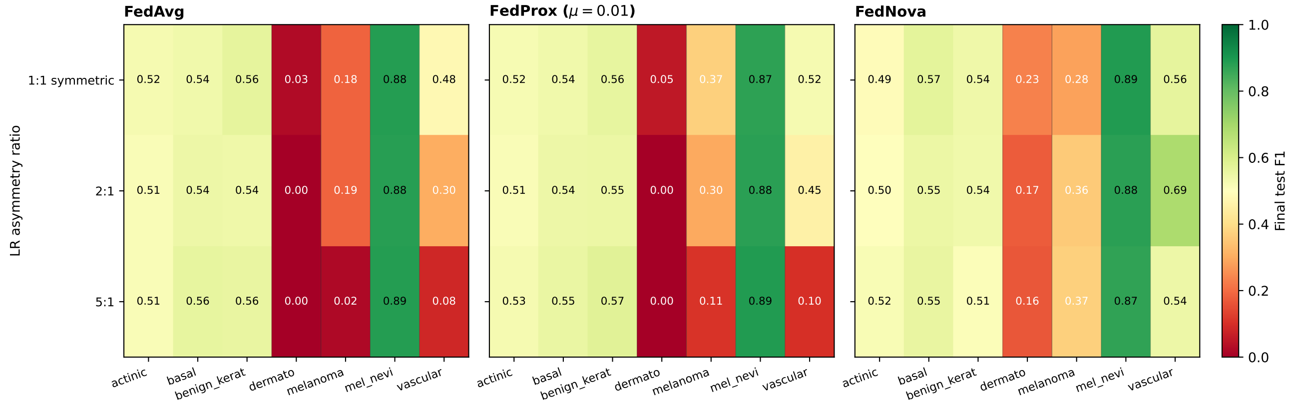
Per-class final F1 across (algorithm × LR ratio) — FedNova preserves rare classes (dermato, melanoma, vascular) where FedAvg/FedProx collapse
