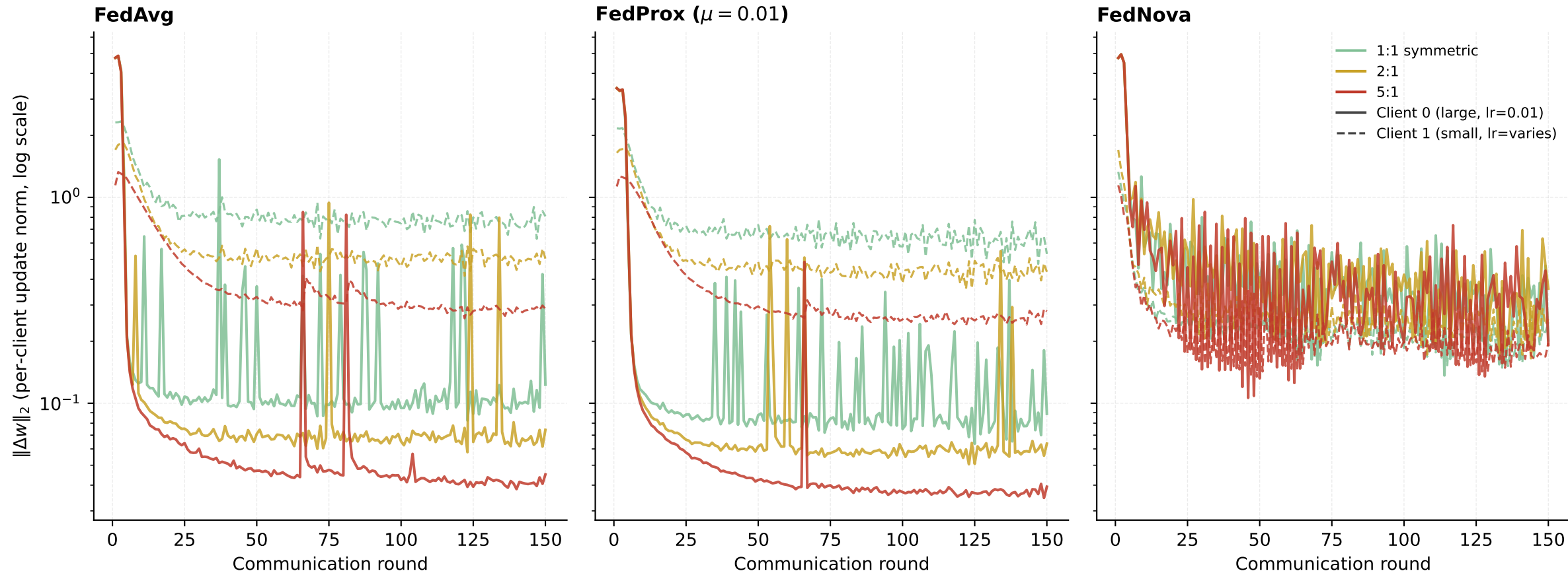
Per-client update-norm trajectories under asymmetric LR — FedNova's Client 1 stays comparable to Client 0 across LR ratios
