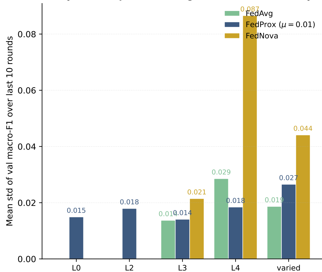
(a) Symmetric protocol — algorithm-level instability by partition
