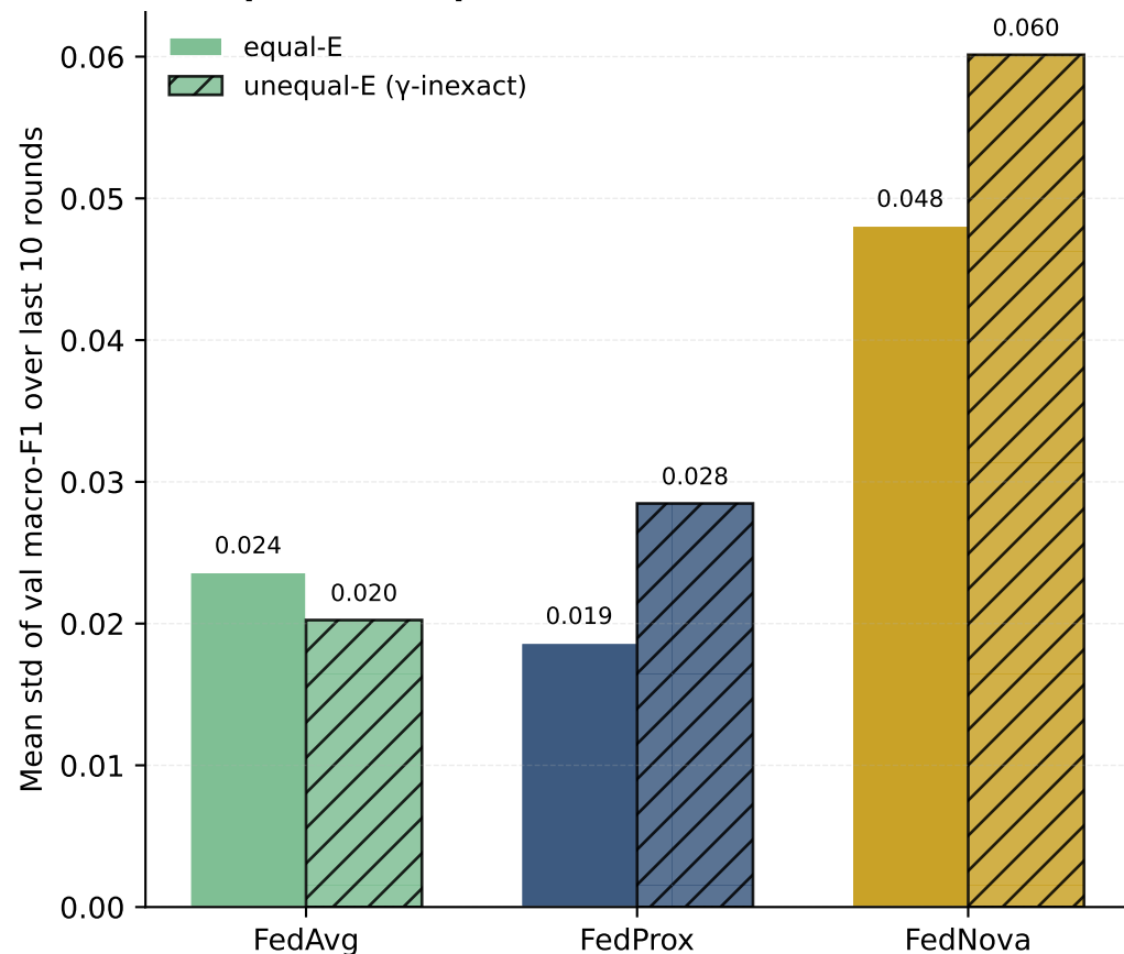
(b) Equal vs unequal-E — FedNova destabilises in its target regime
