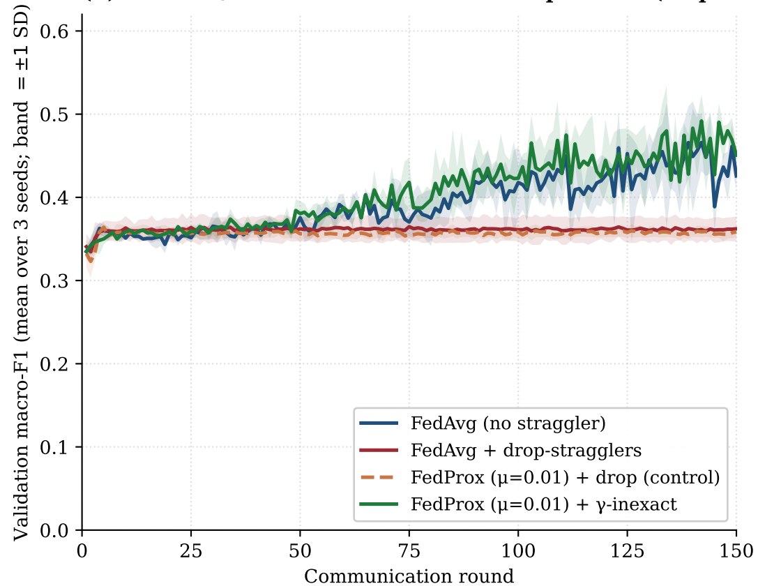
(A) Li 2020 §5.2 — four-condition decomposition ( \Delta up to +0.115)
