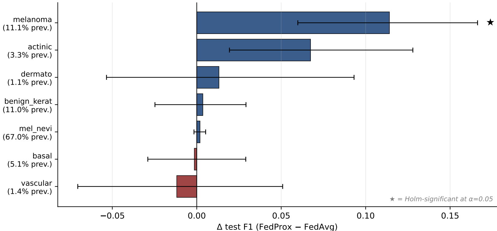
Per-class paired \Delta across 10 seeds (95% bootstrap CI)
