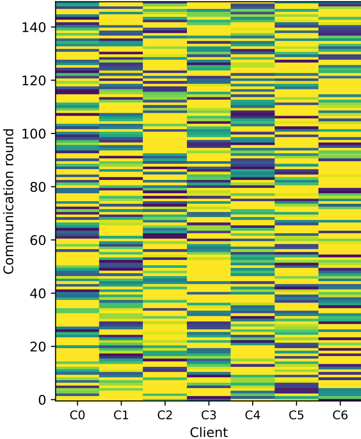
(c) C2 -- random stragglers (primary) 4/7 clients per round, E \sim U\{1..19\}
