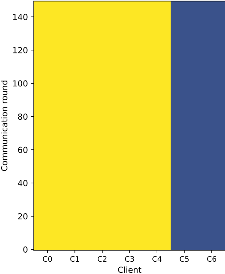
(b) C1 -- fixed stragglers C5, C6 always E = 5
