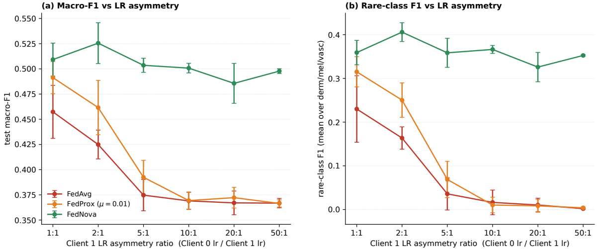
Figure 3.5: Learning-rate asymmetry envelope at L4, n = 3 per cell. Two panels: test macro-F1 and rare-class F1 (mean over dermato, melanoma, vascular) vs the Client 1 LR ratio on a \log_{10} axis from 1:1 to 50:1. FedAvg and FedProx plateau at the rare-class floor; FedNova stays flat across the envelope. Exact macro-F1 values and FedNova deltas are in Table 3.5.
