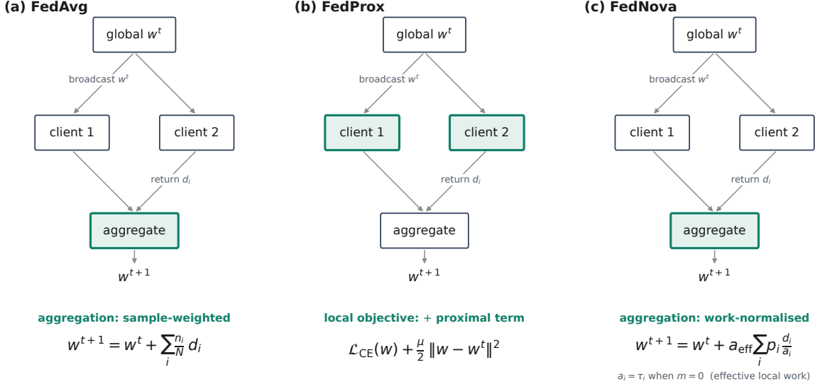
Figure 2.5: Minimal schematic comparison of the three federated optimisers. All three share the same structure — broadcast the global model w^t , train on each client to obtain its update d_i = w_i^{t+1} - w^t , aggregate — and differ only in the highlighted mechanism. FedAvg aggregates locally trained client models by sample-weighted averaging; FedProx keeps that aggregation but adds a proximal penalty to the local objective, discouraging drift from the current global model; FedNova normalises client updates by effective local work before aggregation. The diagram is conceptual; Chapter 3 tests when these mechanisms preserve or lose rare-client signal under statistical and system heterogeneity.
