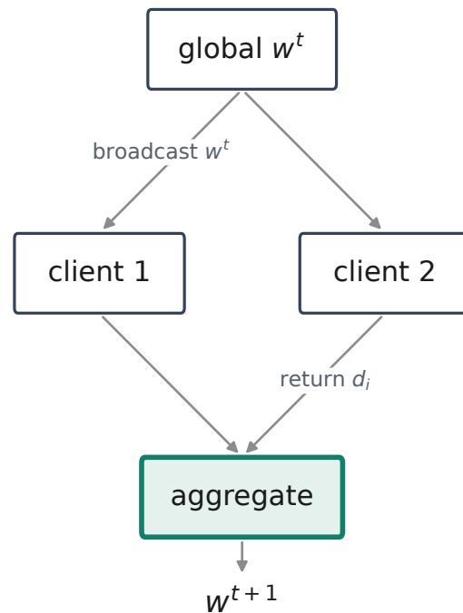
(c) FedNova
