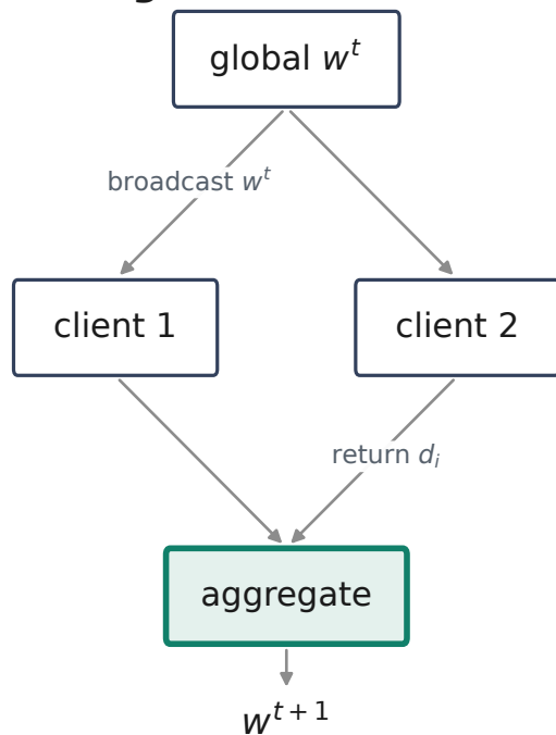
(a) FedAvg
