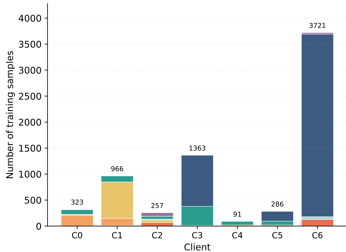
(a) Dirichlet \alpha = 0.1
