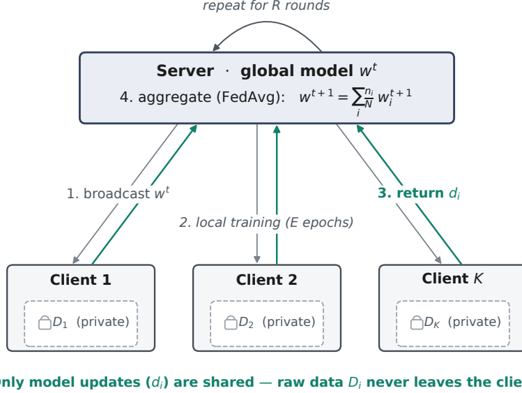
Figure 2.1: Federated learning loop (conceptual; simulated on a single machine in this thesis). Each round the server broadcasts the global model w^t , clients train locally on private data D_i and return model updates d_i (not raw data), and the server aggregates them into w^{t+1} ; the loop repeats for R rounds.
