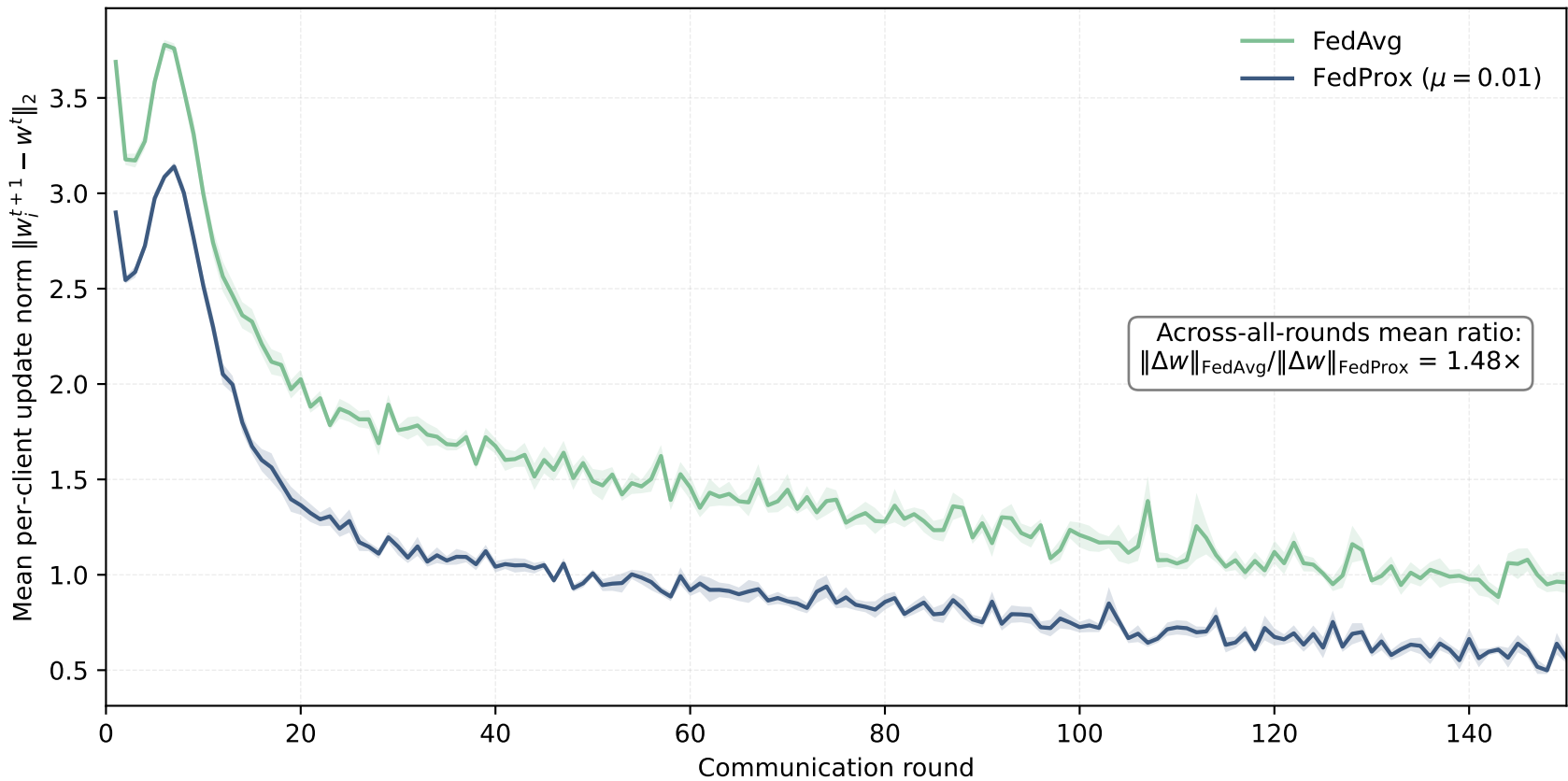
Direct mechanism evidence: per-client update norms across rounds (Flower runtime, engineered partition, mean \pm SEM across seeds)
