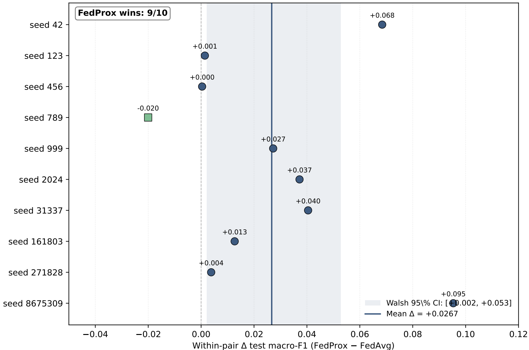
Per-seed paired \Delta (FedProx – FedAvg) with headline mean and CI (Pure-PyTorch primary, n = 10 paired seeds, engineered partition)
