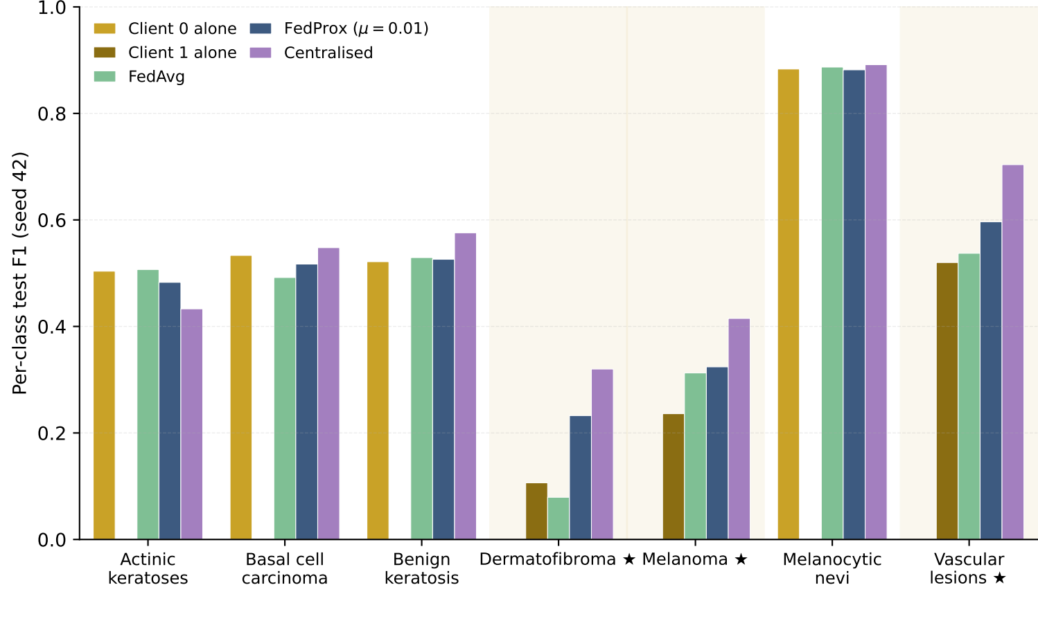
(b) Per-class F1 — ★ = held only by Client 1
