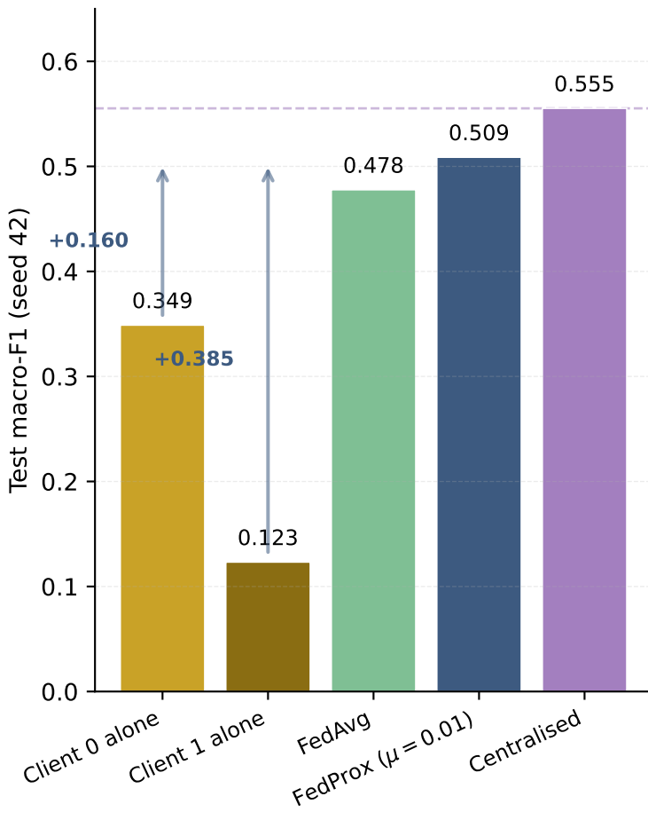
(a) Macro-F1 across configurations
