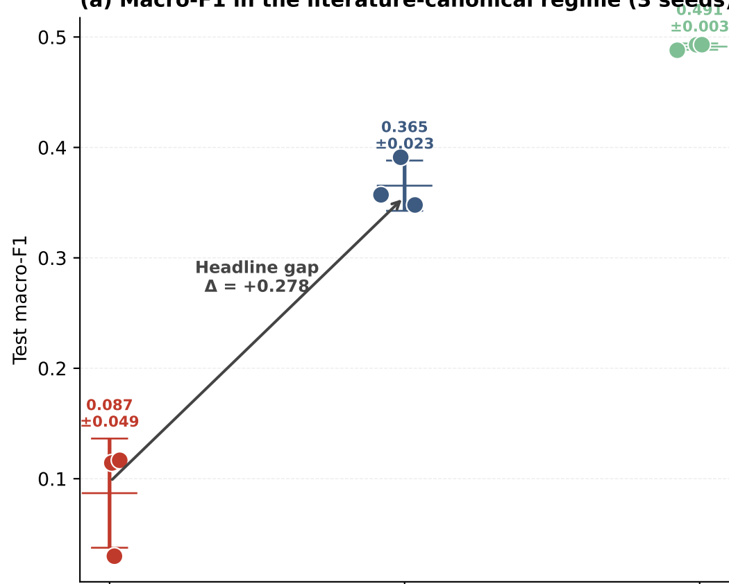
(a) Macro-F1 in the literature-canonical regime (3 seeds)
